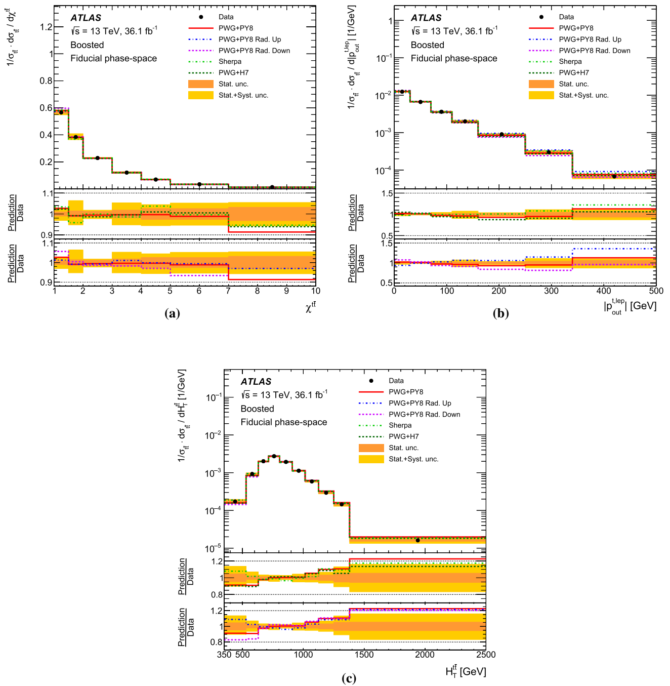
Fig. 41 Particle-level normalised differential cross-sections as a function of a \chi^{if} , b |p_{out}^{tlep}| and c H_T^{if} in the boosted topology, compared with different Monte Carlo predictions. The bands represent the statisti-
