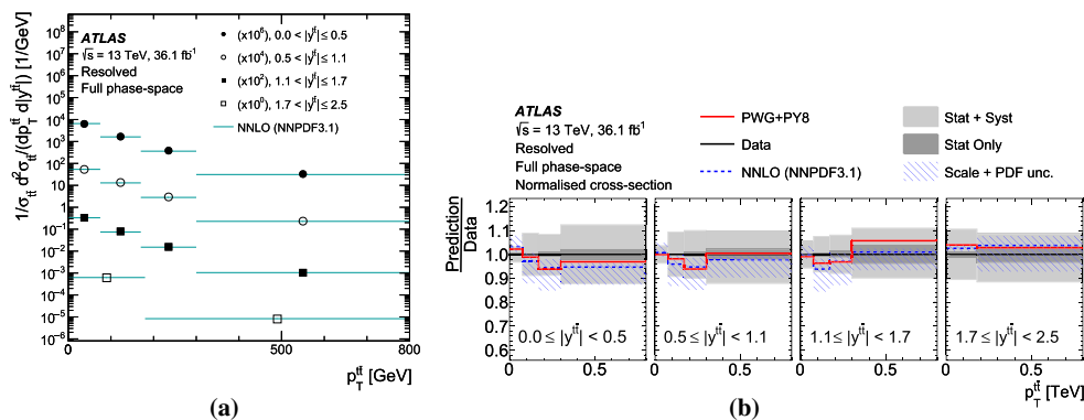
Fig. 61 a Parton-level normalised differential cross-section as a function of p_T^{\text{II}} in bins of |y^{\text{II}}| in the resolved topology compared with the NNLO prediction obtained using the NNPDF3.1 NNLO PDF set. Data points are placed at the centre of each bin. b The ratio of the measured
