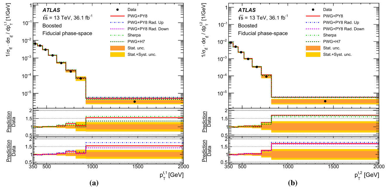
Fig. 38 Particle-level normalised differential cross-sections as a function of the transverse momentum of a the leading and b the subleading top quark in the boosted topology, compared with different Monte Carlo predictions. The bands represent the statistical and total uncertainty in the data. Data points are placed at the centre of each bin. The lower panel shows the ratios of the simulations to data
