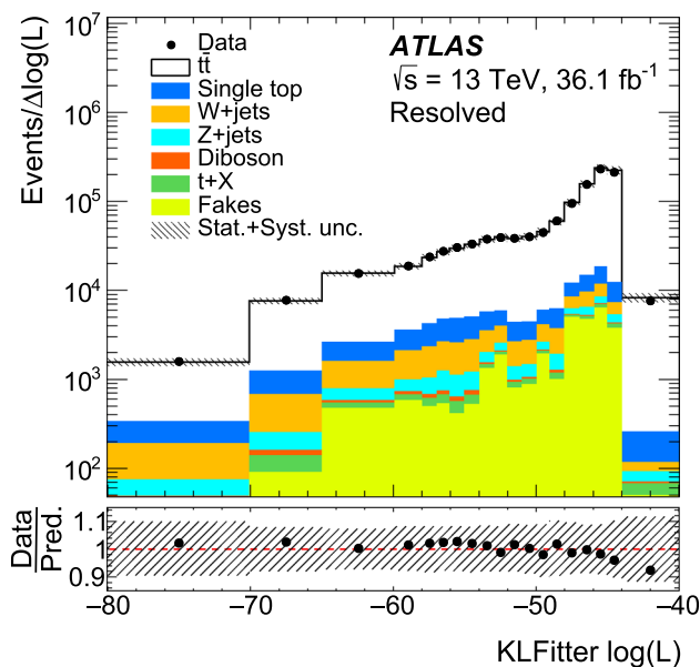
Fig. 5 Distribution in the l + \text{jets} channel of the logarithm of the likelihood obtained from the kinematic fit in the resolved topology. Data distributions are compared with predictions using POWHEG+PYTHIA8 as the t\bar{t} signal model. The hatched area represents the combined statistical and systematic uncertainties in the total prediction, excluding systematic uncertainties related to the modelling of the t\bar{t} events. Underflow and overflow events are included in the first and last bins. The lower panel shows the ratio of the data to the total prediction. Only events with \log L > -52 are considered in the parton-level measurement in resolved topology
