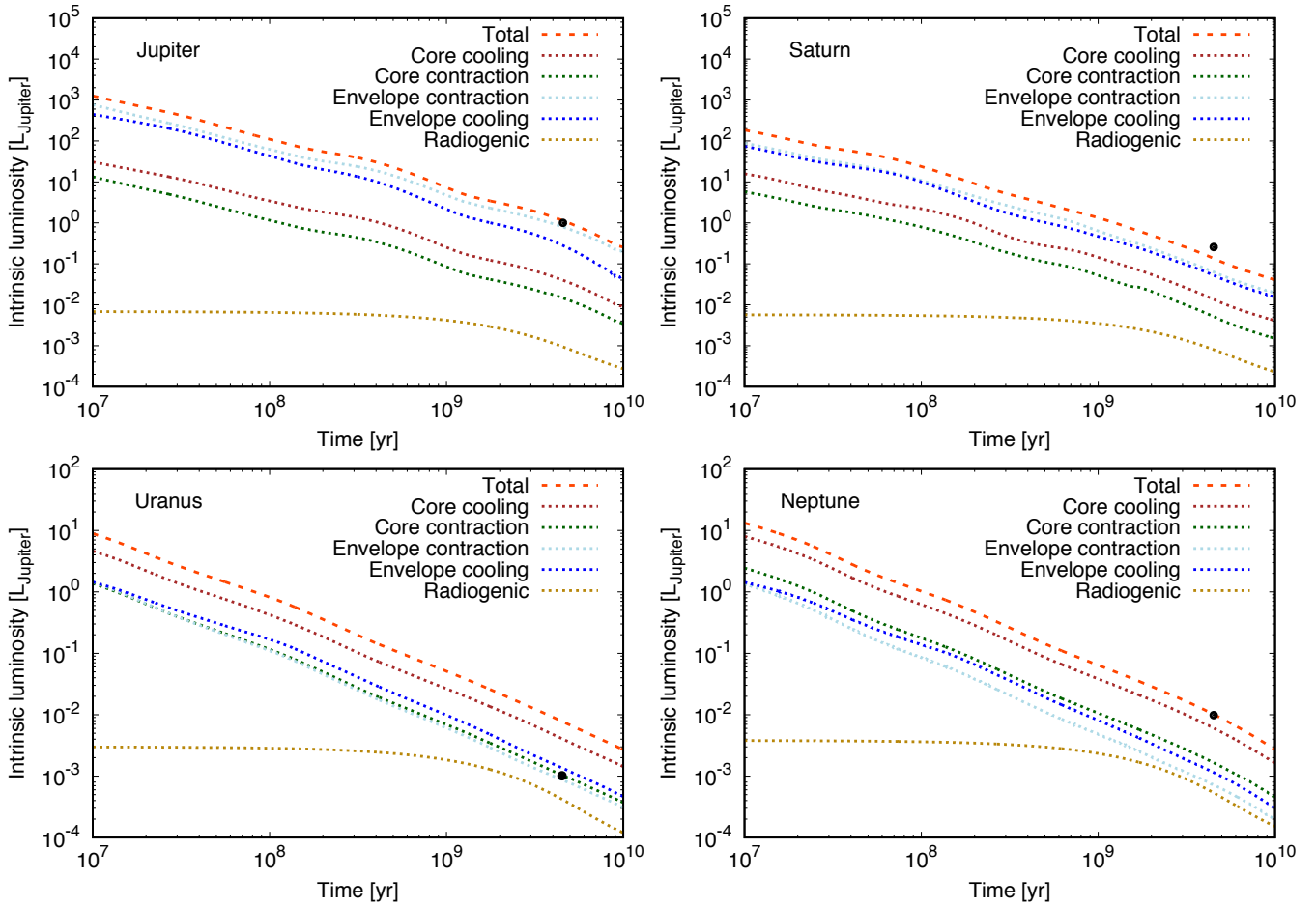
Fig. 1. Temporal evolution of the luminosity of the simplified solar system gas giants. The different contributions to the total luminosity are indicated with colours, the luminosity of today is shown as a black dot.
