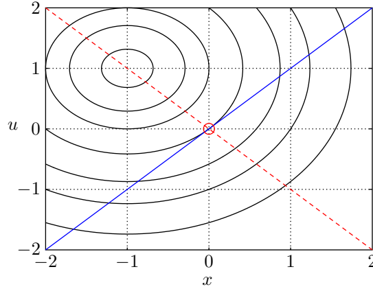
Figure 8.1: Illustration of the steady-states (blue solid line), level sets of \ell (black ellipses), and the additional constraint g_{ad} (red dashed) of the example in Section 8.4. The optimal steady-state (x^e, u^e) = (0, 0) for the undiscounted case is marked with a circle.
