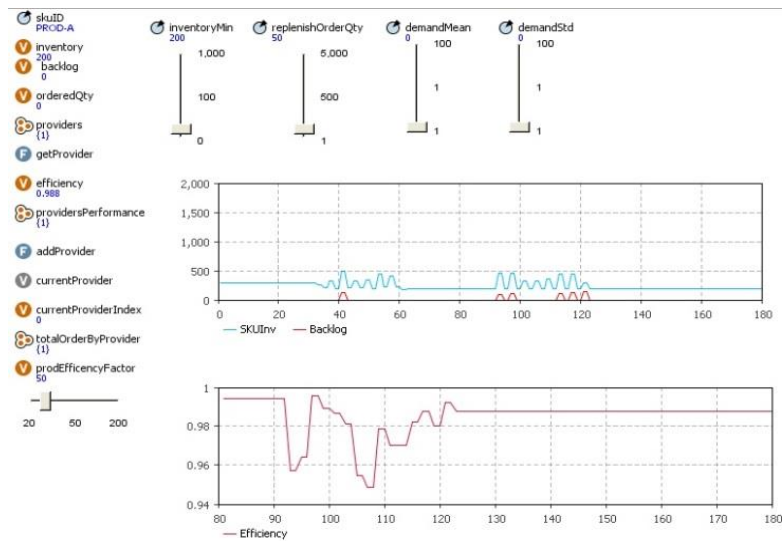
Figure 2: SKU object
