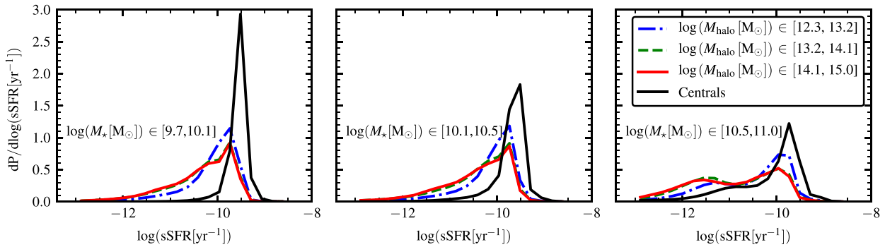
Figure 9. sSFR distributions for galaxies with stellar masses in different mass bins at z = 0 : \log(M_*/[M_\odot]) \in [9.7, 10.1] (left-hand panel), \log(M_*/[M_\odot]) \in [10.1, 10.5] (middle panel), and \log(M_*/[M_\odot]) \in [10.5, 11.0] (right-hand panel). Coloured lines of different style represent satellite galaxies residing in main host DM haloes within different mass ranges, as indicated in the legend. Central galaxies are identified with black thin solid lines; all central galaxies are considered, without any restriction regarding their main host DM haloes. A bimodal distribution emerges only for the most massive galaxies considered, with a break at \text{sSFR} = 10^{-10.7} \text{ yr}^{-1} , a value in good agreement with the one adopted by Brown et al. (2017) and slightly higher than the one identified from the observational catalogue constructed by W12.
