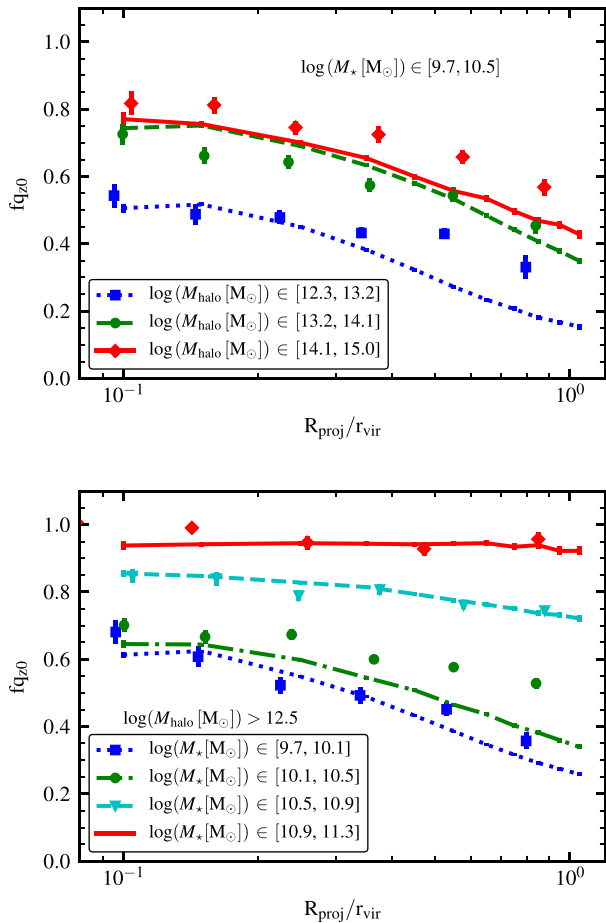
Figure 12. Fraction of quenched satellite galaxies ( \text{sSFR} < 10^{-10.7} \text{ yr}^{-1} ) in model \text{SAG}_{\beta 1.3} at z = 0 as a function of the projected halo-centric distance normalized with the virial radius of the main host halo. Satellites are binned according to their main host halo mass (top panel) and stellar mass (bottom panel). Model results are shown by different lines; error bars show the 68 per cent Bayesian confidence interval estimated following Cameron (2011). Only satellites within the stellar mass range \log(M_*/[M_\odot]) \in [9.7, 10.5] are considered in the top panel and with main host halo mass \log(M_{\text{halo}}[M_\odot]) > 12.5 in the bottom one. Such selection is done following W12 for comparison purposes. Their data are represented by different symbols according to the different stellar or halo mass ranges.
