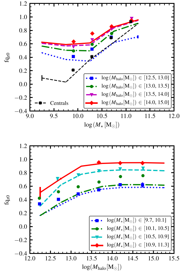
Figure 11. Same as Fig. 10 for galaxies generated with model \text{sAG}_{\beta 1.3} . The general agreement with observations is rather good except for the underprediction of the quenched fraction for galaxies within the mass range \log(M_*, [M_\odot]) \in [10.1, 10.5] .
