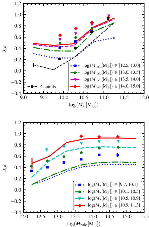
Figure 10. Fraction of quenched galaxies ( s\text{SFR} < 10^{-10.7} \text{ yr}^{-1} ) in \text{sAG} model at z = 0 as a function of stellar mass (top panel) and main host halo mass (bottom panel). Satellite galaxies are binned according to their main host halo or stellar mass, and are represented by coloured lines of different style, as indicated in the legend. Central galaxies, represented by a thin black dashed line, are only included in the top panel without making any distinction to the mass of the halo they reside in. Error bars show the 68 per cent Bayesian confidence interval estimated following Cameron (2011); they are hardly visible for the satellite population. These fractions are compared to those obtained by W12 (different symbols associated with different line styles). The calibrated \text{sAG} model underpredicts the fraction of quenched galaxies. Only the most massive galaxies, those in the stellar mass range \log(M_*, [M_\odot]) \in [10.9, 11.3] within DM host haloes with masses M_{\text{halo}} \gtrsim 10^{14} M_\odot achieve a quenched fraction similar to the observed one. This lack of general agreement is related to the underpredicted SFRD at high redshifts, as discussed in Section 6.1. The value \beta = 1.99 that regulates the redshift dependence of the reheated and ejected mass in \text{sAG} model is too high and produces a shift of the SF activity to lower redshifts not leaving enough time for quenching.
