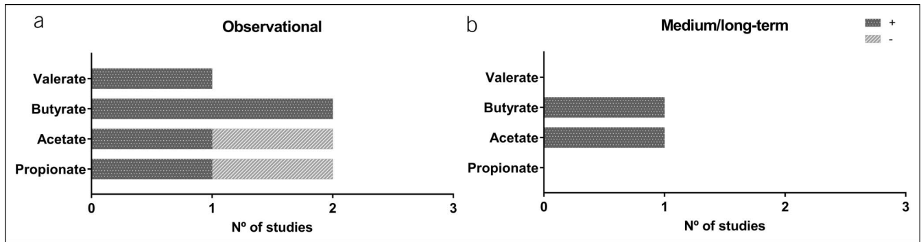
Figure 3. Summary of the main findings of the present review with respect to short-chain fatty acids (SCFAs), by study design. Panel (a) represents the main results of all observational studies ( n = 2 ). Panel (b) shows the main results of the medium/long-term studies ( n = 1 ). The dark grey bars (+) indicate the number of studies showing a positive association between levels of physical activity or cardiorespiratory fitness and SCFAs, or a positive effect for an exercise intervention. The light grey bars (–) indicate a negative association between levels of physical activity or cardiorespiratory fitness and SCFAs.
