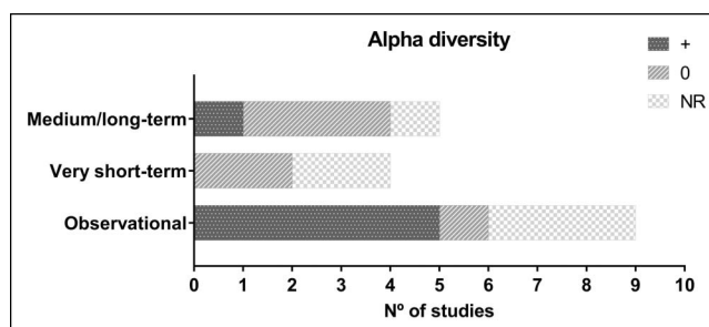
Figure 2. Influence of exercise on alpha diversity by study design. The dark grey bars (+) indicate the number of studies showing a positive association between physical activity or cardiorespiratory fitness and bacterial alpha diversity. The light grey bars (0) represent the number of studies showing no influence of physical activity or cardiorespiratory fitness on alpha diversity. The light grey and white bars (“NR”) indicate the number of studies that reported no results in this respect. NR, no results.
