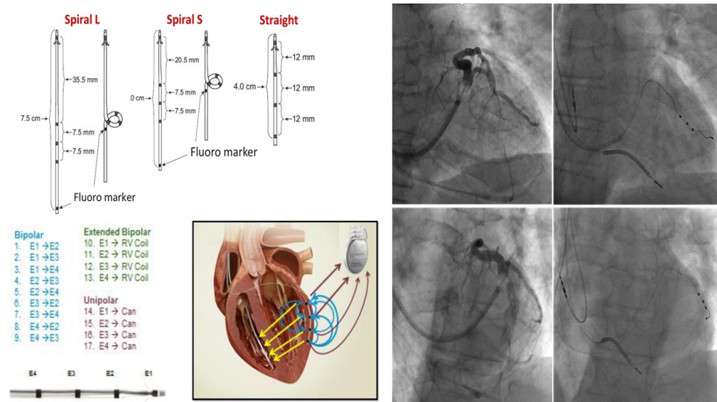
Figure 1: Acuity Spiral long (L), Spiral Short (S) and Straight lead models, with the 17 programmable pacing vectors (including unipolar pacing for CRT-Ds). Spacing between the distal (E1) and most proximal (E4) electrode is comparable between the Acuity Straight and Spiral S leads, and is similar
