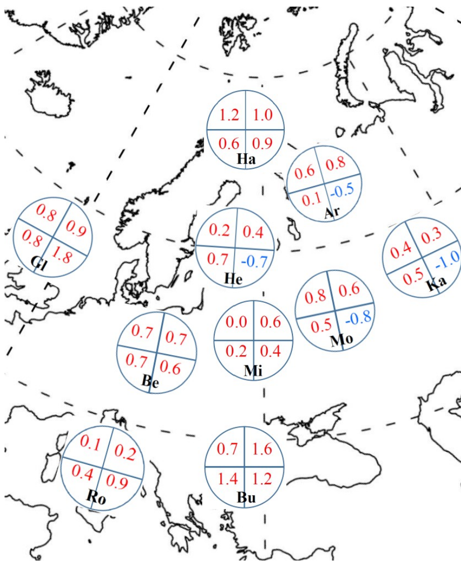
Figure 11. Differences in winter (DJFM) mean air temperature ( ^{\circ}\text{C} ) at 1 km height between the periods 1998-2015 and 1979-1997 in cases of airmass origins in the northwest, northeast, southeast, and southwest (noted in corresponding quadrants of circles) for Archangelsk (Ar), Berlin (Be), Bucharest (Bu), Glasgow (Gl), Hammerfest (Ha), Helsinki (He), Kazan (Ka), Minsk (Mi), Moscow (Mo), and Rome (Ro).
