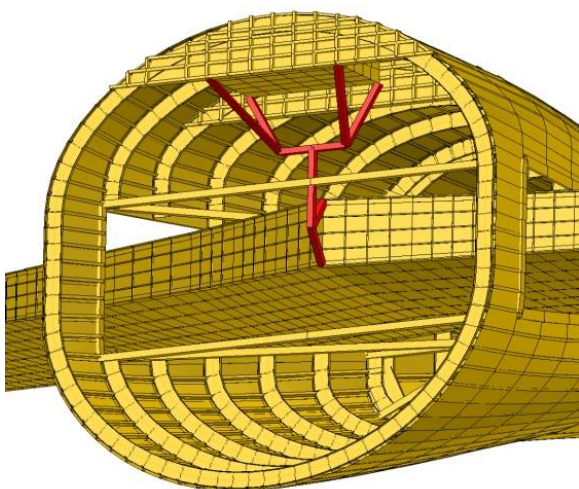
Figure 9: Empennage attachment.
