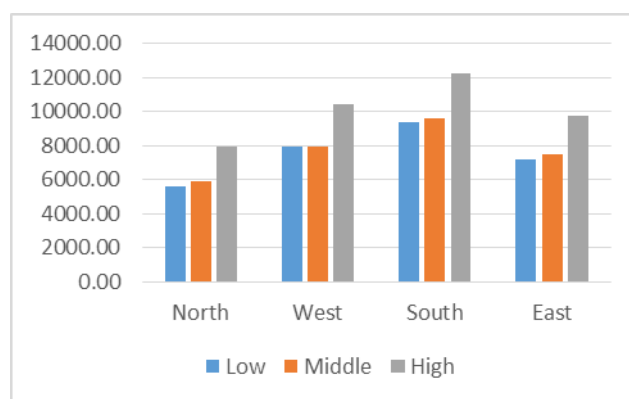
Fig .5 Average Illuminance Level on centralized atrium's floor level (Low) and vertical walls. Chart derived from numerical table of (Yunus, Ahmad, & Zain-ahmed, 2011)
