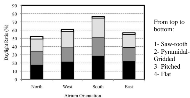
Fig .6 Daylight Ratio at different atrium vertical wall orientation under overcast skies for different roof aperture types (Yunus et al., n.d.)
