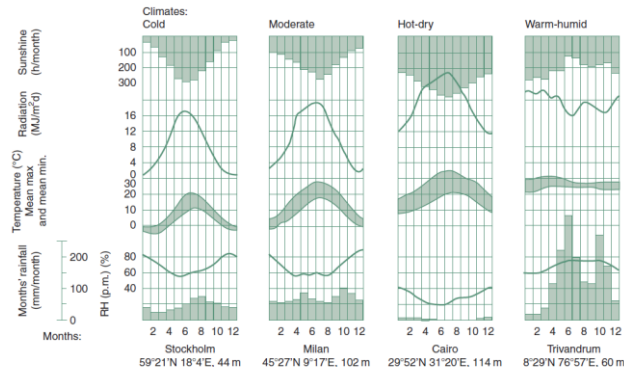
Fig. 28 Composite (simplified) climate graphs for the four basic types (Szokolay, 2014)
