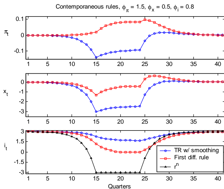
Figure 12: Dynamic paths: truncated Taylor rule with smoothing vs truncated first-difference rule
