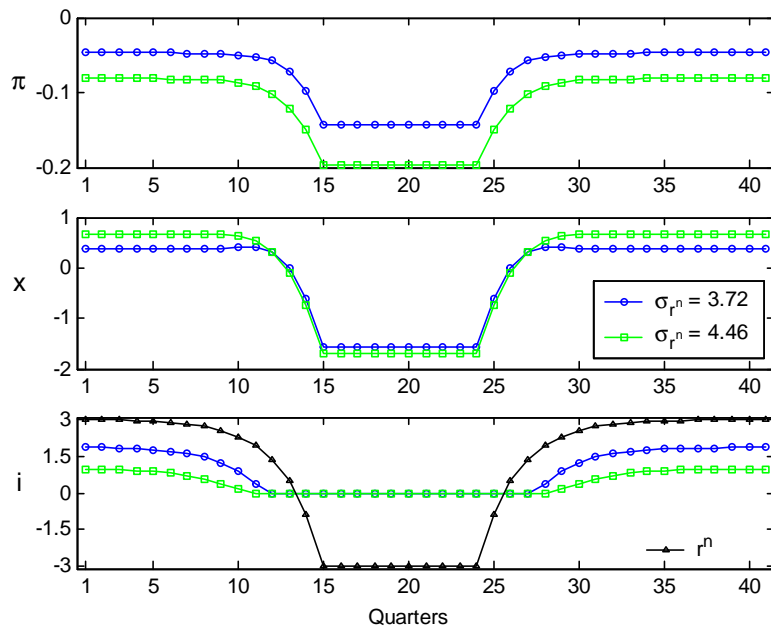
Figure 14: Sensitivity of ODP to \sigma(r^n)
