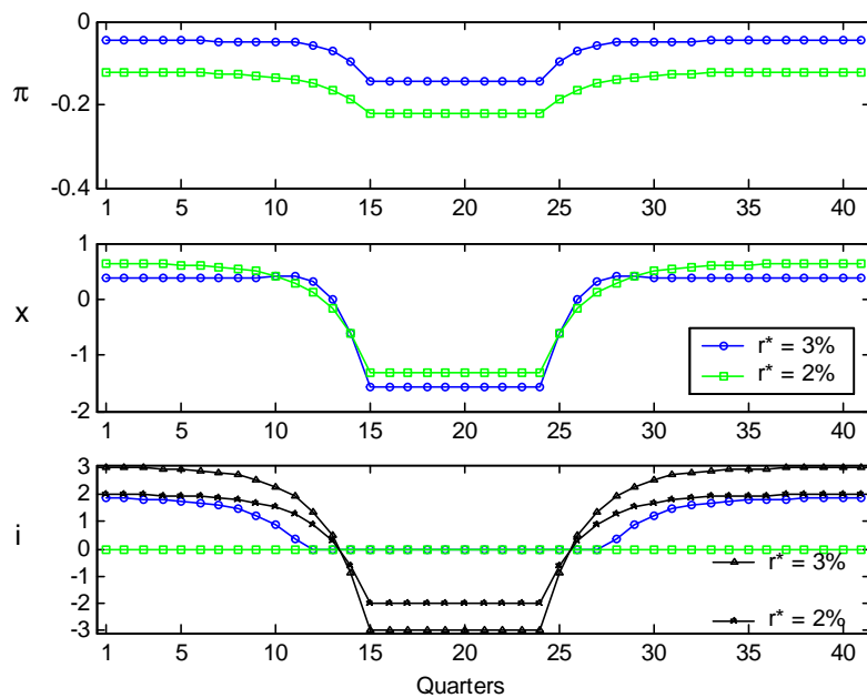
Figure 19: Sensitivity of ODP to r^*
