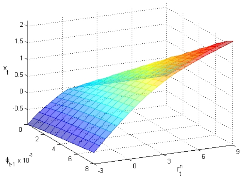
Figure 5: Optimal commitment policy (output gap)
