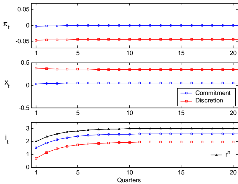
Figure 7: Impulse-responses to a small shock: commitment vs discretion
