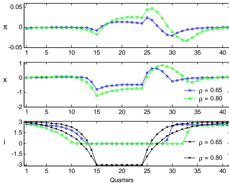
Figure 15: Sensitivity of OCP to \rho
