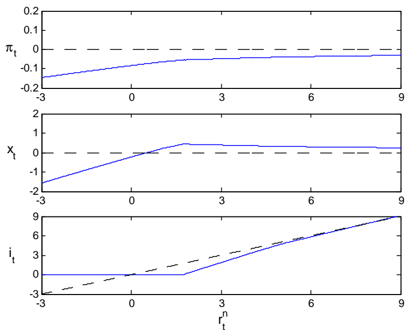
Figure 3: Optimal discretionary policy in the stochastic case
