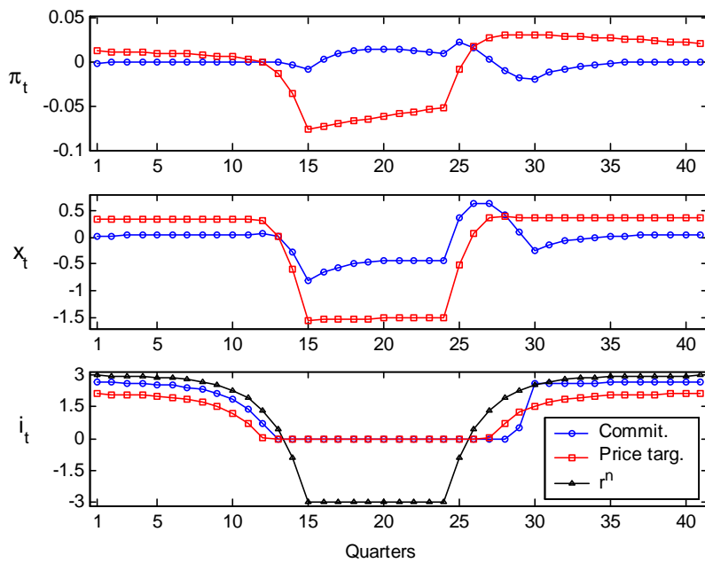
Figure 10: Dynamic paths under constant price level targeting
