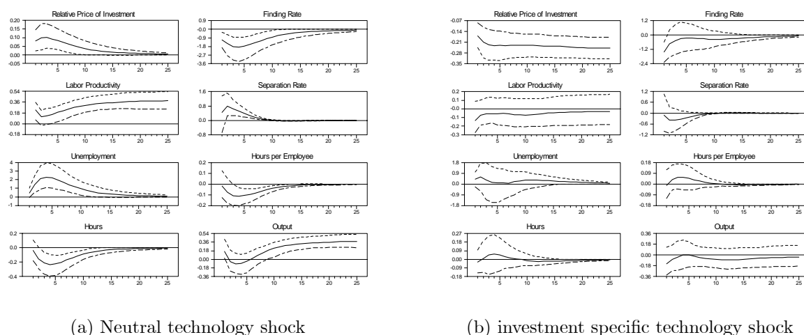
Figure 11: The sample period is 1955:I-1973:I. The VAR has eight lags and contains six variables: the rate of growth of the relative price of investment, the rate of growth of labour productivity, the (logged) job finding rate, the (logged) job separation rate, the (logged), unemployment rate (logged), and the (logged) aggregate number of hours worked per capita. Dotted lines represent the 5% and 95% quantiles of the distribution of the responses simulated by bootstrapping 500 times the residuals of the VAR. The continuous line corresponds to median estimate from bootstrap replications.
