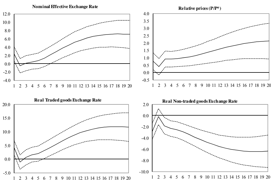
Figure 9. Decomposition of the REER in the US
