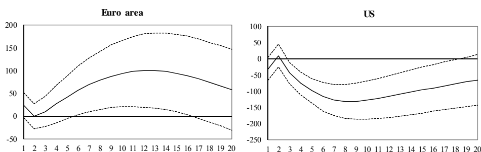
Figure 10. Effects of government spending on the short-term nominal interest rate spreads
