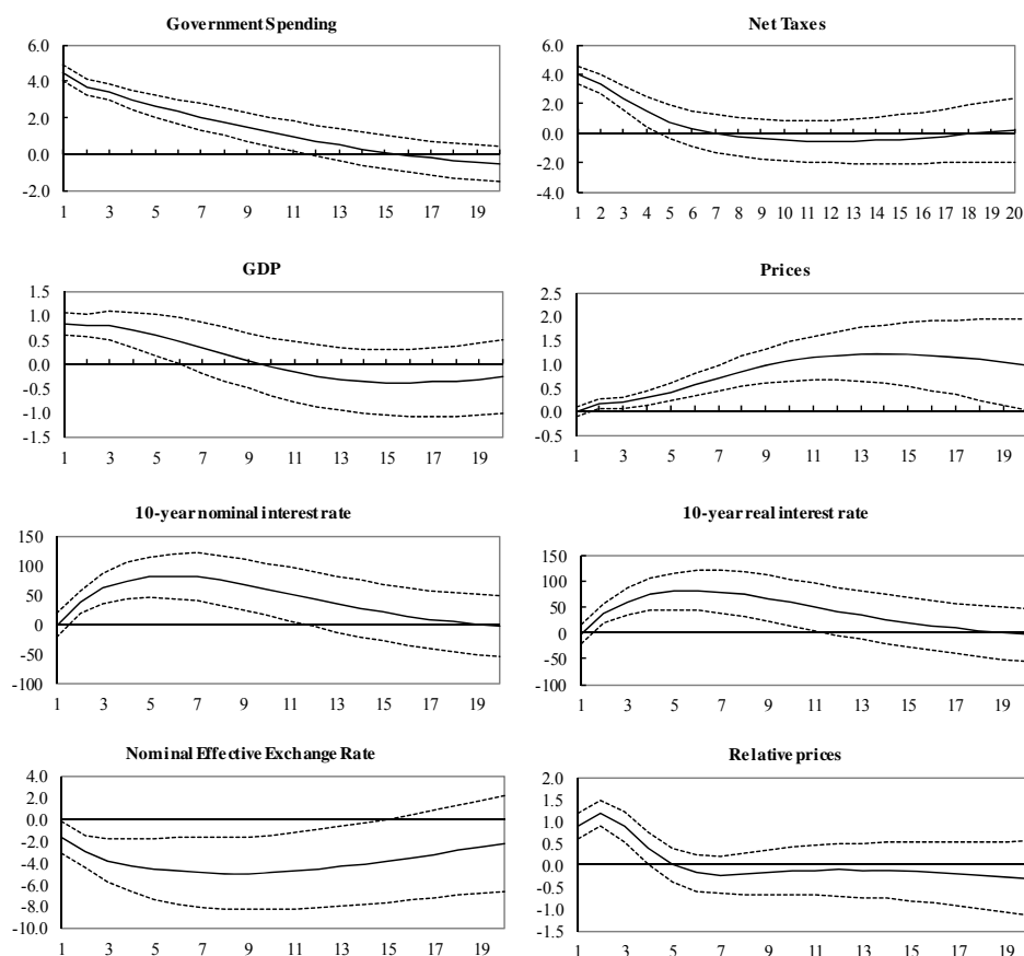
Figure 2. Responses to an increase in government spending in EMU: VAR with nominal effective exchange rates and relative prices
