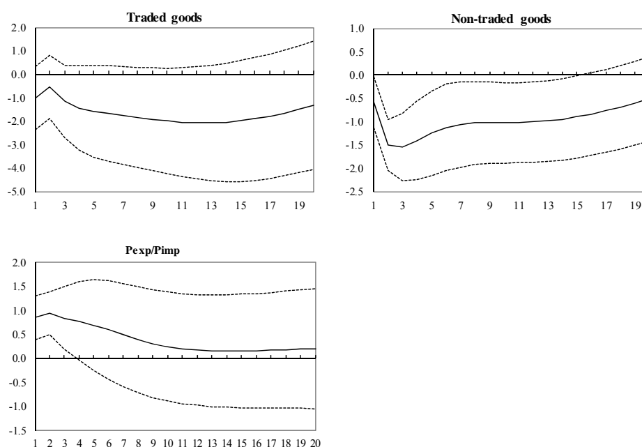
Figure 3. Responses of real exchange rates of traded and non-traded goods to a spending shock in EMU
