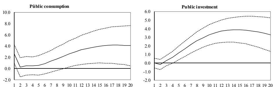
Figure 8. Responses of the REER to different government spending components in the US
