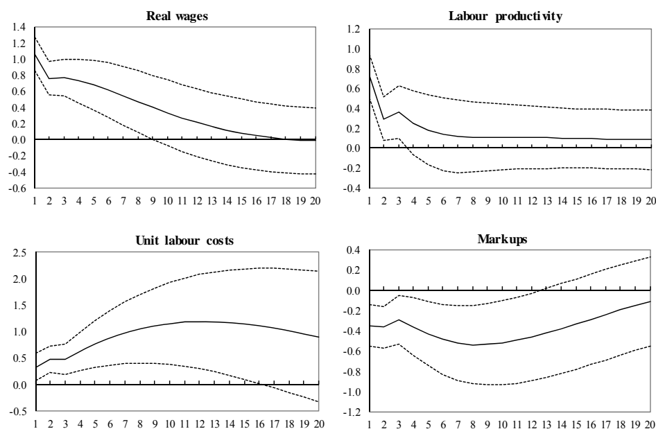
Figure 4. Effects of government spending on costs, productivity and mark-ups in EMU
