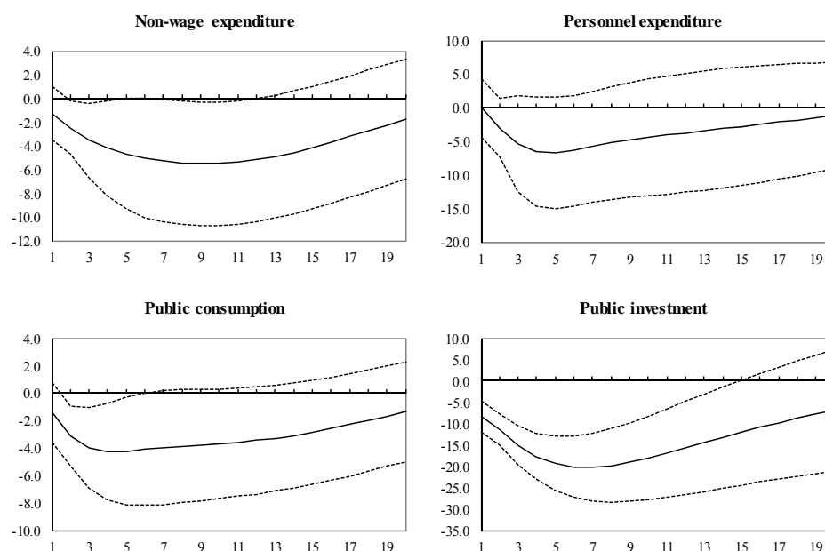
Figure 6. Responses of the real effective exchange rate to shocks to different government spending components in EMU
