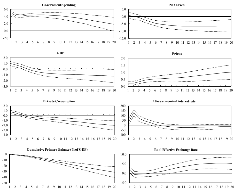
Figure 7. Responses to an increase in government spending in the US
