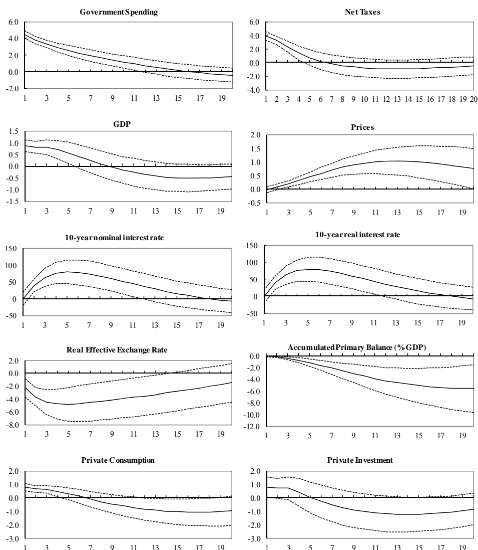
Figure 1. Responses to an increase in government spending by 1% of GDP in the EMU: Baseline VAR
