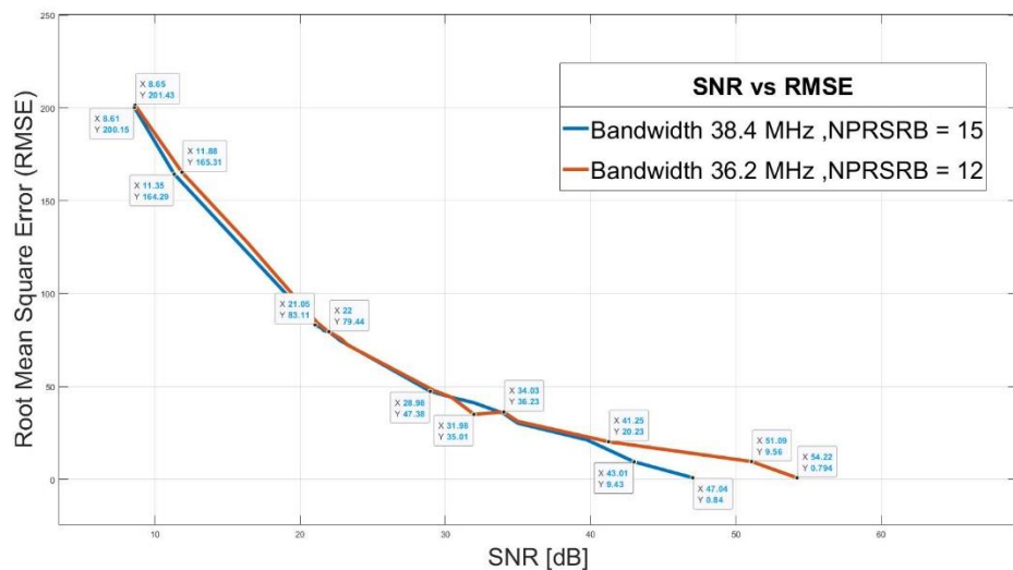
Figure 15: SNR vs RMSE with a Bandwidth of 38.4 MHz and 36.2 MHz
