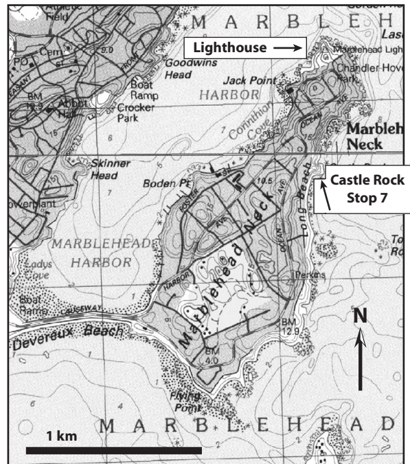
Figure 21. On the left is an outcrop photograph of dark, plagioclase-phyric vitrophyre and light agglomerate (with dark vitrophyre clasts) at Castle Rock. A penny is visible for scale. On the right is a location map for Marblehead Neck from the Marblehead North and Marblehead South 7.5-minute quadrangles.
