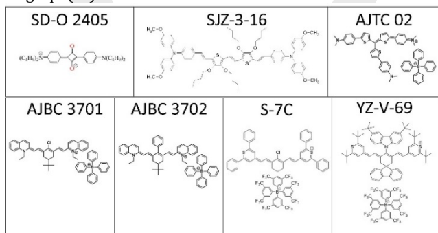
Figure 5. Chemical structures of the molecular systems under study. All the molecules are approximated as linear symmetric molecules ignoring the small permanent dipole moment perpendicular to the long axis except AJTC 02, which has no permanent dipole moment.
