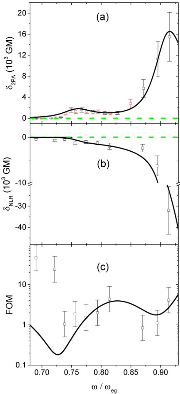
Figure 9 (a) 2PA cross sections of SD-O 2405 measured via dual-arm Z-scans (black squares) and two-photon induced fluorescence (red squares) plotted along with the fit from the quasi 3-level model. (b) NLR cross sections measured via dual-arm Z-scans plotted with the quasi 3-level model prediction of the dispersion of NLR. (c) Experimental FOM along with the prediction. The green dashed line in (a) and (b) shows \delta=0 .
