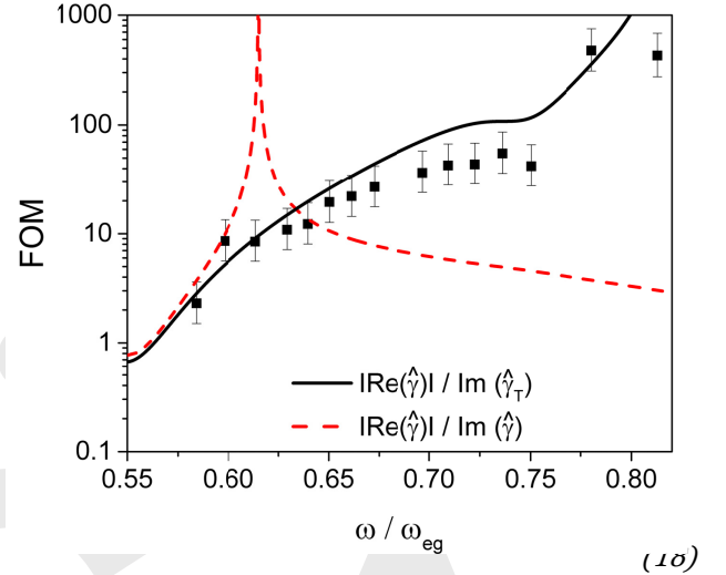
Figure 3. FOM for YZ-V-69 from the experimental data in Figure 2 along with the calculated result from Eqn. (17). The solid black line is the result when the imaginary component of the N-terms have been excluded from Im(\hat{\gamma}) . The dashed red line is the result when the imaginary component of the N-terms are included in Im(\hat{\gamma}) .
