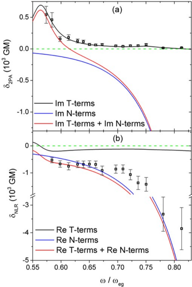
Figure 2. (a) 2PA spectrum along with quasi 3-level essential-state model fit for YZ-V-69 (molecular structure shown in Figure 5) dissolved in carbon tetrachloride. (b) The experimentally determined \delta_{NLR} spectrum and predicted fits. The solid black line, blue line, and red line in (a) and (b) represent the T-terms, N-terms, and their sum, respectively. The green dashed line in (a) and (b) shows \delta = 0 .
