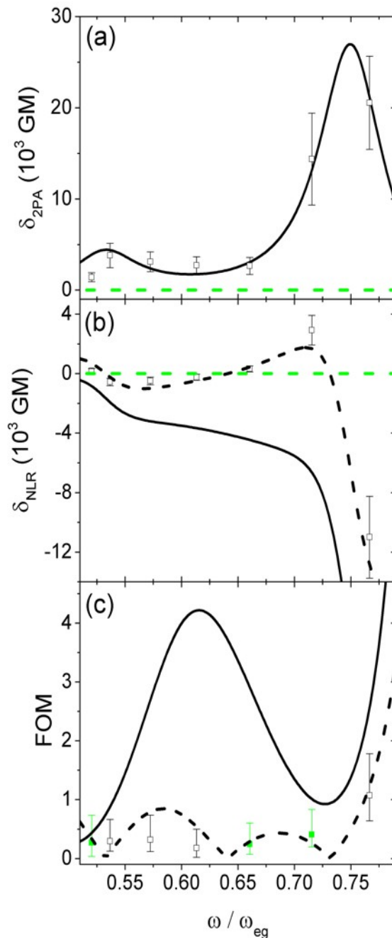
Figure 12. (a) 2PA cross sections of AJTC 02 measured via Z-scans plotted along with the fit from the quasi 3-level model to obtain the parameters. (b) NLR cross sections measured via dual-arm Z-scans plotted with the quasi 3-level model prediction of the dispersion of NLR. (c) Experimental FOM along with the prediction. The black dashed lines in (b) and (c) represent the predicted NLR dispersion and FOM, respectively, using a smaller value of \mu_{ge} than that listed in
