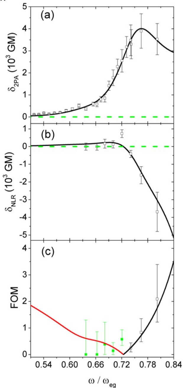
Figure 7 (a) 2PA cross sections of SJZ-3-16 measured via two-photon induced fluorescence plotted along with the fit from the quasi 3-level model [53]. (b) NLR cross sections measured via white-light continuum Z-scans plotted with the quasi 3-level model prediction of the dispersion of NLR. (c) Experimental FOM along with the prediction. The solid red line in (c) gives the FOM where the quasi 3-level model predicts \delta_{NLR} > 0 and the solid black line shows the FOM where \delta_{NLR} < 0 . Note that the green data points in (c) represent measurements of positive or “zero” NLR. The green dashed line in (a) and (b) gives \delta=0 .
