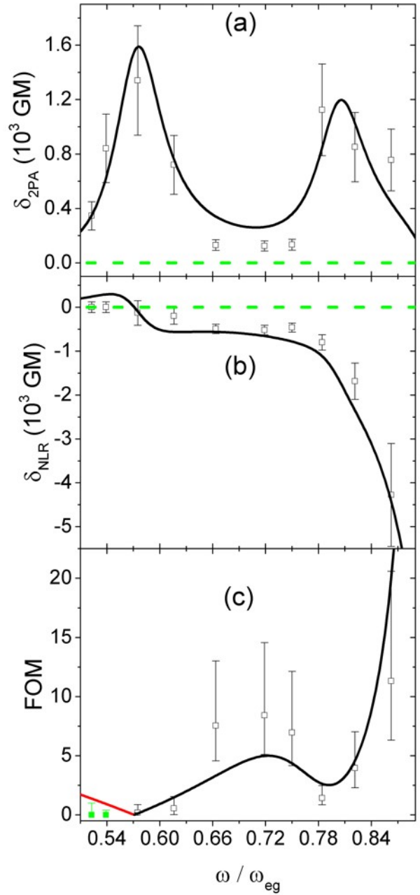
Figure 10(a) 2PA cross sections of AJBC 3702 measured via Z-scans plotted along with the fit from the quasi 3-level model. (b) NLR cross sections measured via Z-scans plotted with the quasi 3-level model prediction of the dispersion of NLR. (c) Experimental FOM along with the prediction. The solid red line in (c) gives the predicted FOM where the quasi 3-level model gives \delta_{NLR} > 0 and the solid black line shows the predicted FOM where \delta_{NLR} < 0 . The green data points in (c) represents a measurement of zero NLR (i.e. too small to measure). The green dashed line in (a) and (b) shows \delta=0 .
