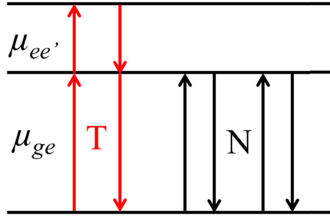
Figure 1. Schematic of the quasi 3-level model for centrosymmetric molecules showing the origin of N and T-terms and indicating the various level couplings. The transitions shown are the perturbation pathways for a centrosymmetric molecule, corresponding to the “T-terms” and “N-terms” described in the text. Due to parity selection rules, the only nonzero transition dipole moments are \mu_{ge} and \mu_{ee'} , as described in the text.
