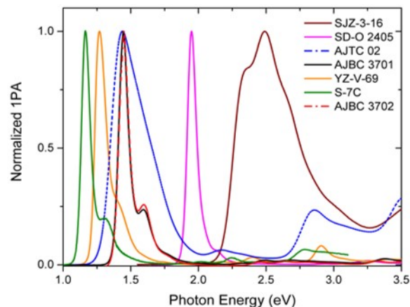
Figure 6. Normalized linear optical absorption spectra for the molecules in Figure 5. SJZ-3-16 is dissolved in tetrahydrofuran, SD-O 2405 in toluene, AJTC 02 in dichloromethane, AJBC 3701 and AJBC 3702 in dimethylformamide, YZ-V-69 in carbon tetrachloride, and S-7C in chloroform.
