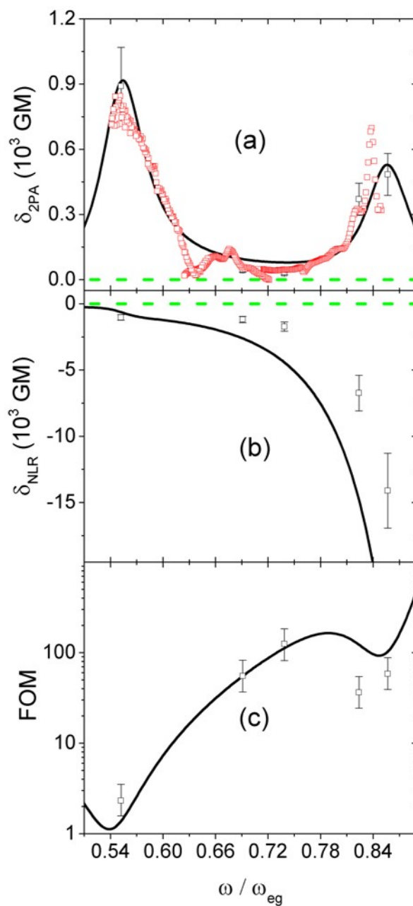
Figure 8 (a) 2PA cross sections of S-7C measured via Z-scans (open black squares) and non-degenerate 2PA (open red squares) plotted along with the fit from the quasi 3-level model to obtain the parameters. (b) NLR cross sections measured via Z-scans plotted with the quasi 3-level model prediction of the dispersion of NLR. (c) Experimental FOM along with the prediction. The green dashed line in (a) and (b) shows \delta=0 .
