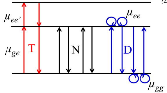
Figure B1. Schematic of the quasi 3-level model for non-centrosymmetric molecules. The perturbation pathways include dipolar ("D") terms in addition to the N and T-terms. Dipole moments \mu_{gg} and \mu_{ee} , correspond to transitions with the same initial and final state, which are allowed in non-centrosymmetric molecules as described in the text.
