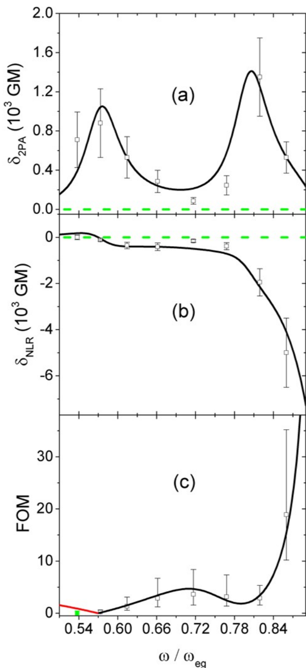
Figure 11 (a) 2PA cross sections of AJBC 3701 measured via dual-arm Z-scans plotted along with the fit from the quasi 3-level model. (b) NLR cross sections measured via dual-arm Z-scans plotted with the quasi 3-level model prediction of the dispersion of NLR. (c) Experimental FOM along with the prediction. The solid red line in (c) shows the predicted FOM where the quasi 3-level model predicts \delta_{NLR} > 0 and the solid black line shows the predicted FOM where \delta_{NLR} < 0 . The green data point in (c) represents a measurement of zero NLR. The green dashed line in (a) and (b) give \delta = 0^8 .
