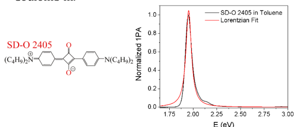
Figure 4. The structure and normalized linear optical absorption (1PA) of the squaraine dye (SD-O 2405) dissolved in toluene. The solid red line is a Lorentzian fit to extract the width of the ground-state transition.
