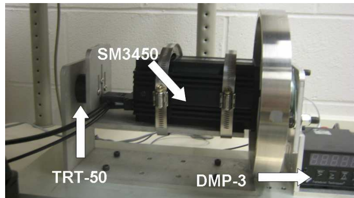
Figure 3.6 AFIT Torque Stand
