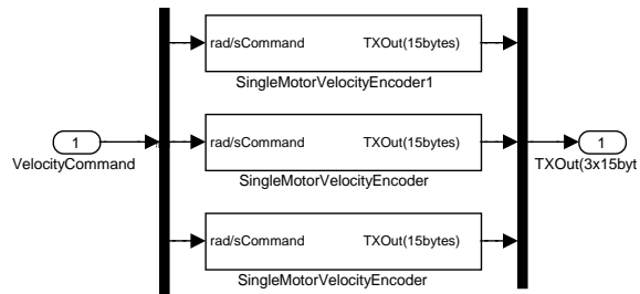
Figure D.10 Reaction Wheel Velocity Encoder and Position Query
