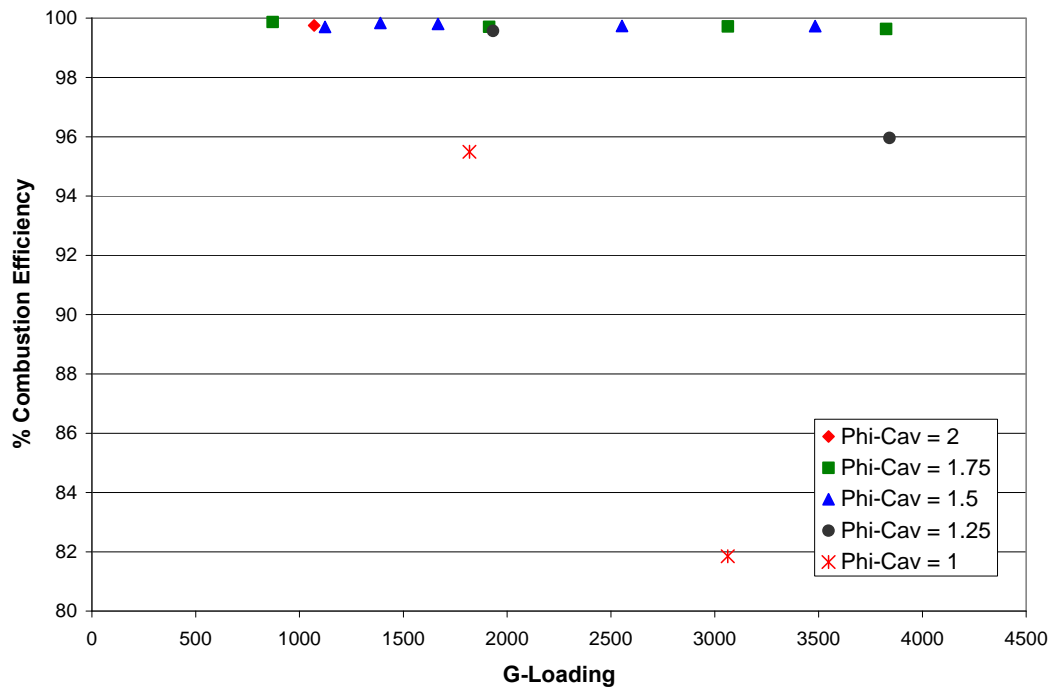
Figure 46. Efficiencies of UCC in the JP-8 CW configuration as a function of g-loading
