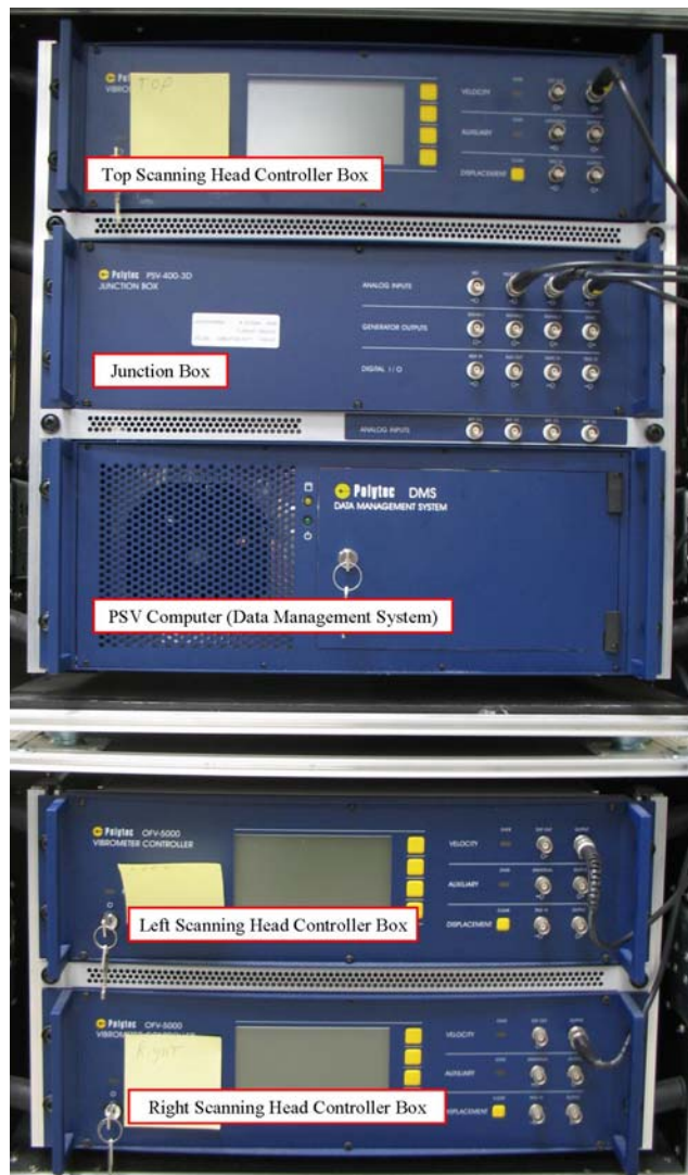
Figure 6: PSV Controllers, Junction Box, and Data Management System
