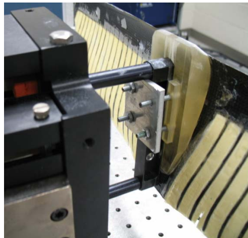
Figure 10: MAV Wing Support
