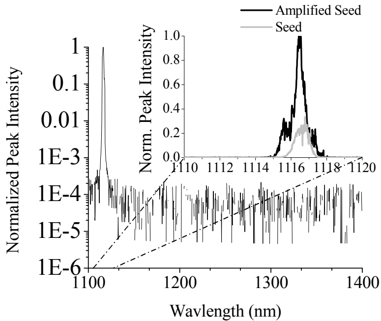
Figure 39. Spectra of the output of the FSR geometry of the RFA beam combiner. Inset uses a linear y axis scale; otherwise the y axis uses a logarithmic scale.
