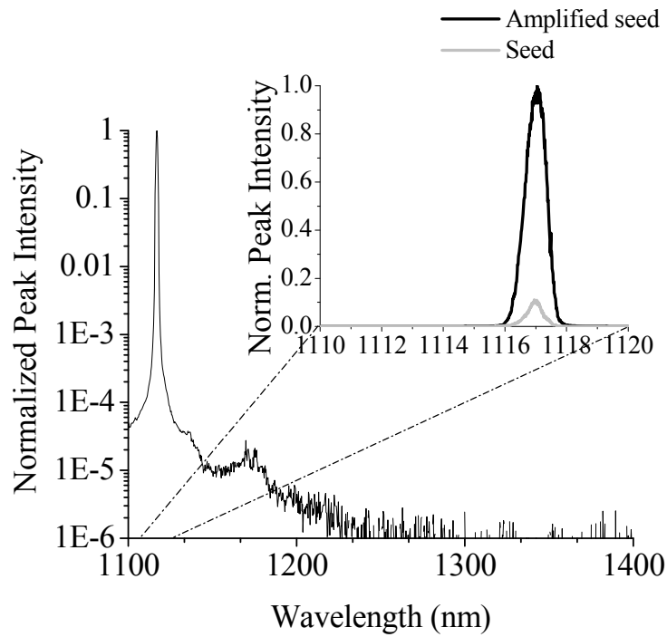
Figure 39. Spectra of the output of the FSR geometry of the RFA beam combiner. Inset uses a linear y axis scale; otherwise the y axis uses a logarithmic scale.
