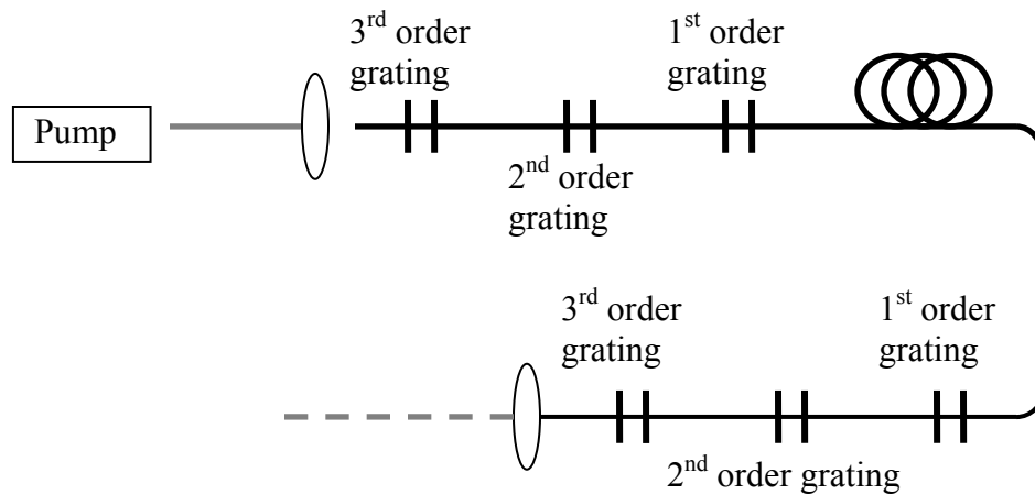
Figure 57. Diagram of a cascaded RFL.
