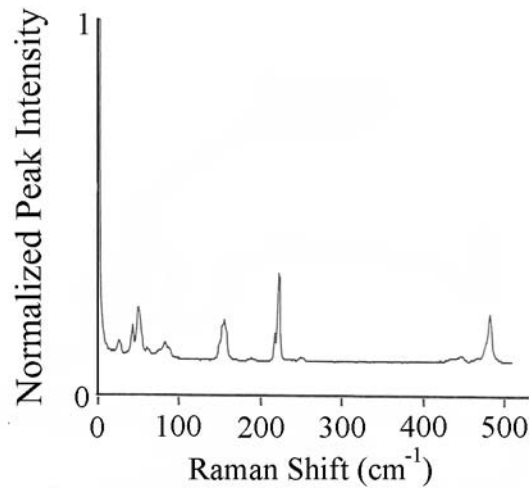
Figure 4. The Raman spectrum of sulfur, normalized to the peak intensity of the input probe beam [33].
