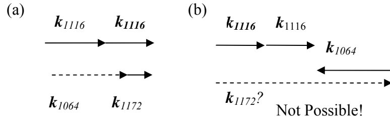
Figure 27. The phase-matching condition of FWM can only be satisfied in the FSRS geometry (a) and not in the BSRS geometry (b) because conservation of energy dictates that \mathbf{k}_{1172} must have a smaller magnitude than \mathbf{k}_{1116} .
