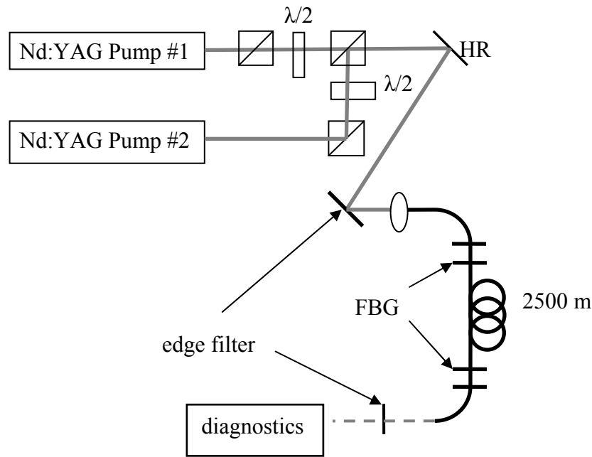
Figure 68. Experimental setup of an RFL beam combiner.
