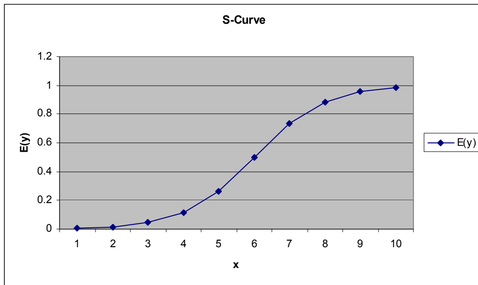
Figure 3-10. Monotonically Increasing S-Curve with 0 \leq E(y) \leq 1
