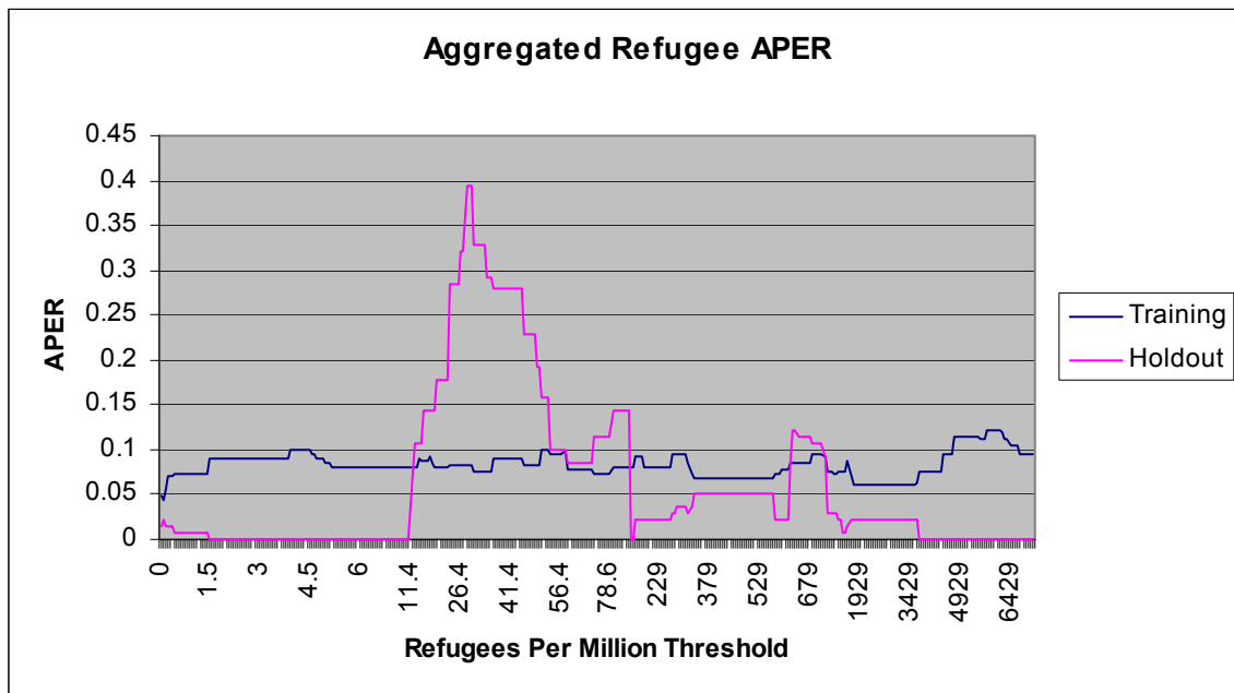
Figure 4-8. Aggregated APER for PCA Scores with Logistic Regression
