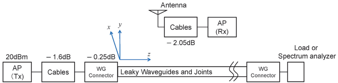
Figure 20. Experimental configuration.
