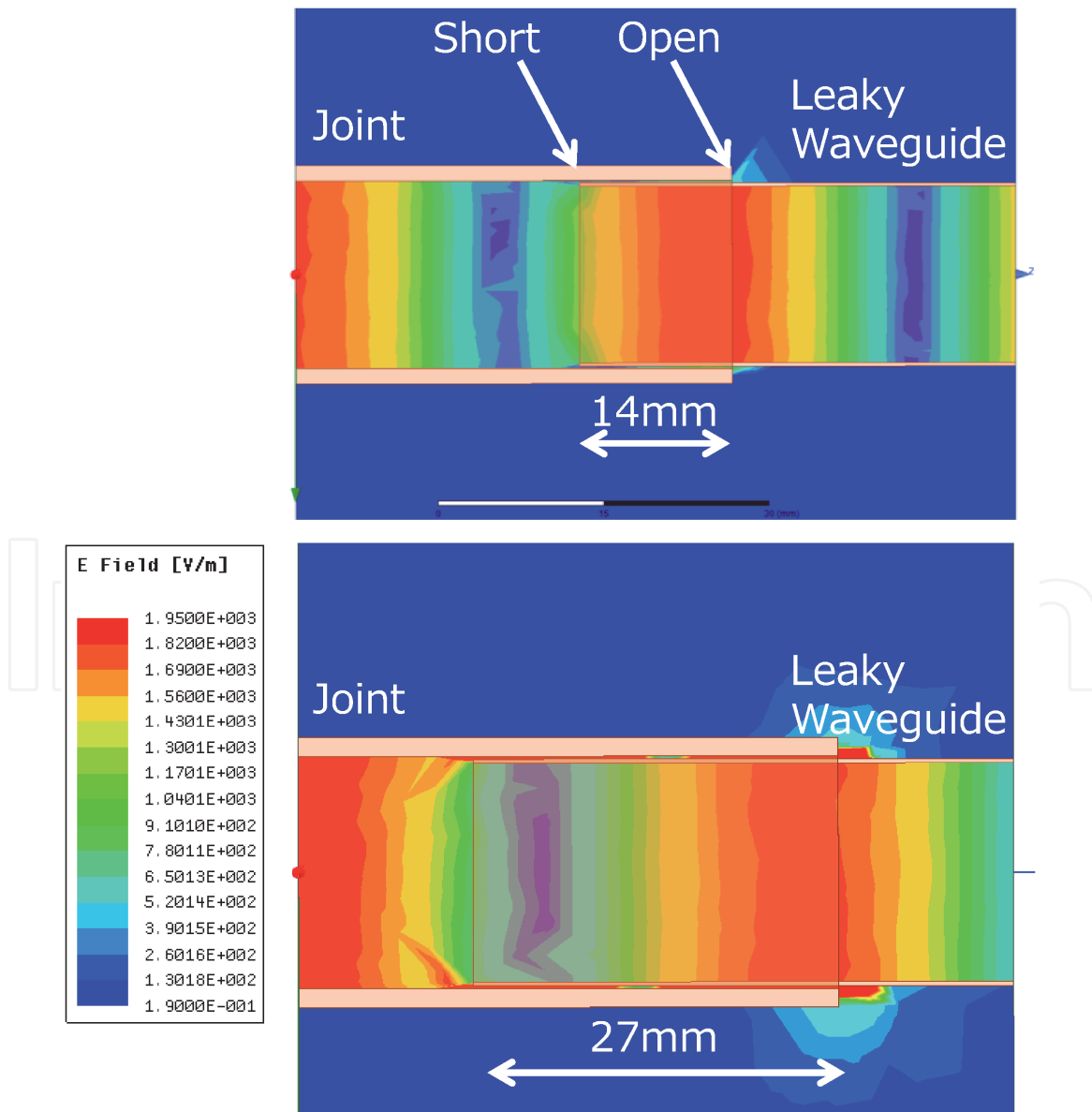
Figure 19. Radiation from the joint (electric field).
