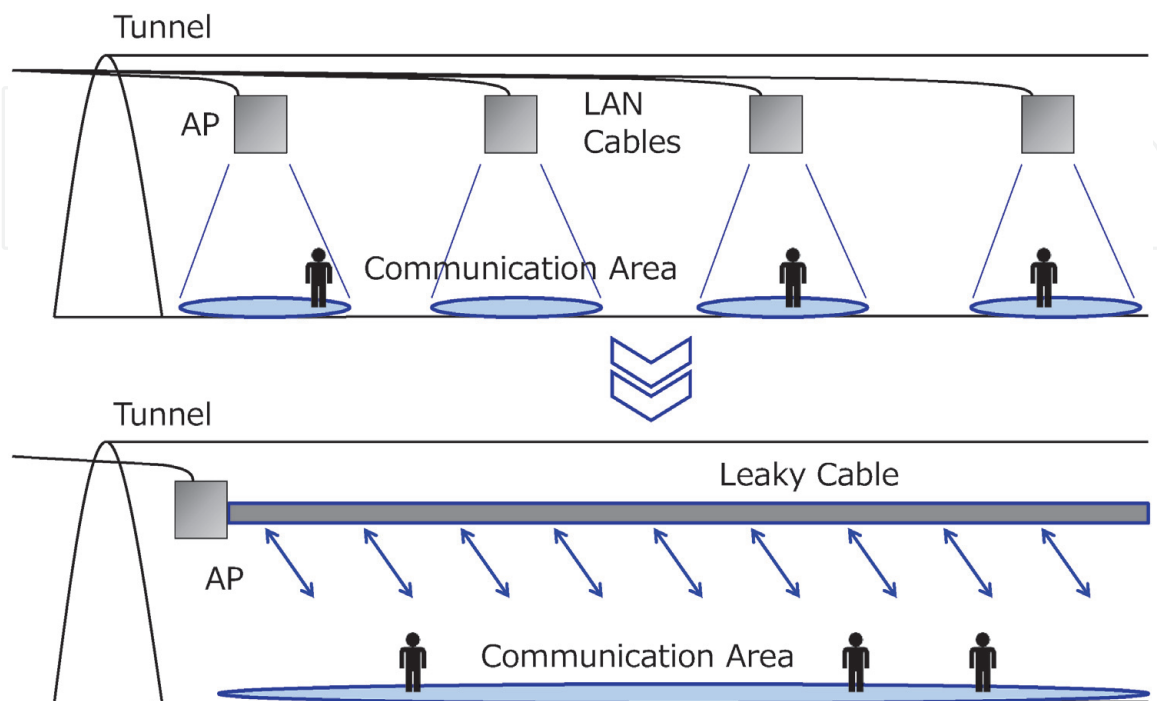
Figure 1. Wireless communication system using a leaky cable.
