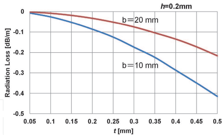
Figure 16. Relationship between slit width and radiation.
