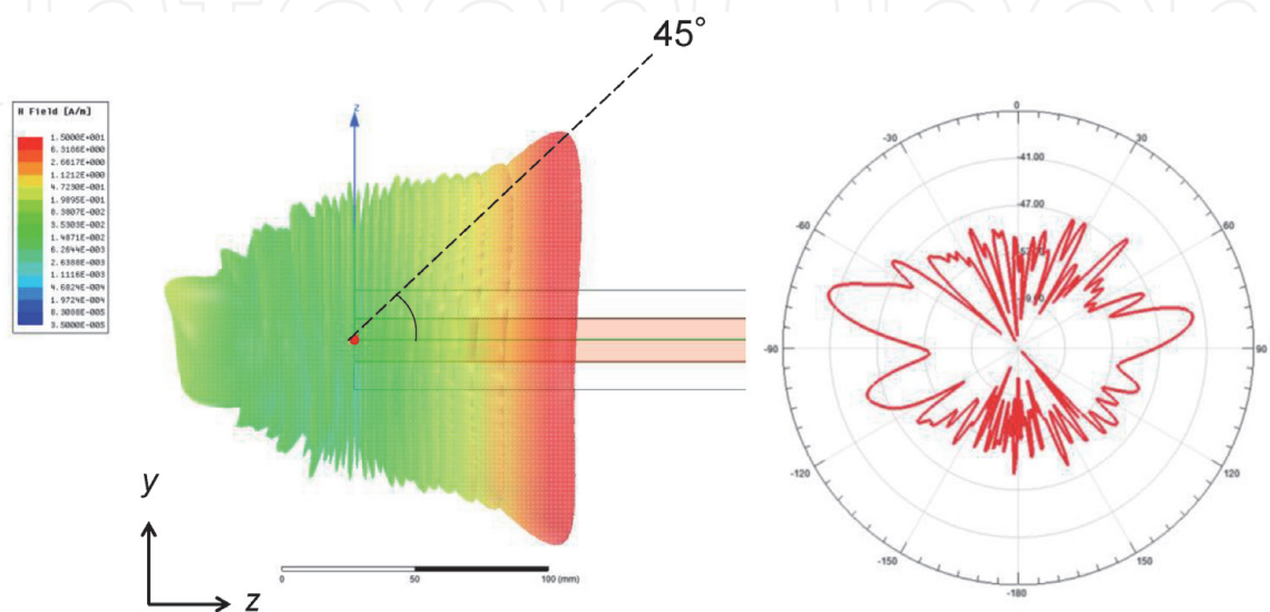
Figure 11. Far-field radiation pattern and gain (y-z plane).
