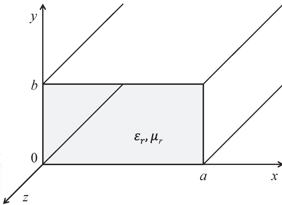
Figure 3. Rectangular waveguide.
