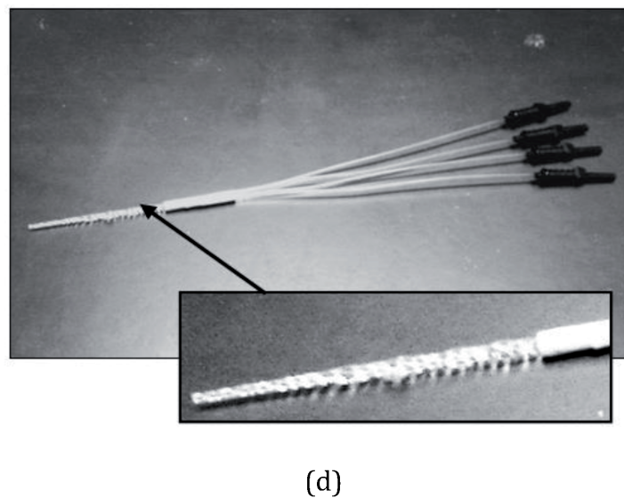
Figure 2. Fabrication process of fused tapered coupler: (a) configuration, (b) twisting and (c) fusion and (d) prototype of the 1 \times 4 handmade coupler fabricated by fused tapering technique.
