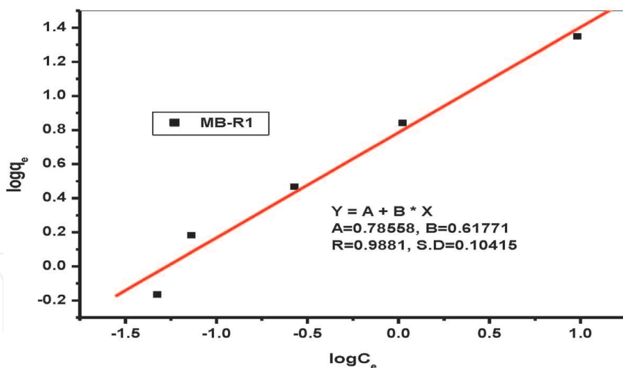
Figure 13. Freundlich model isotherm plot for the sorption of MB onto the synthesized sorbent R1.
