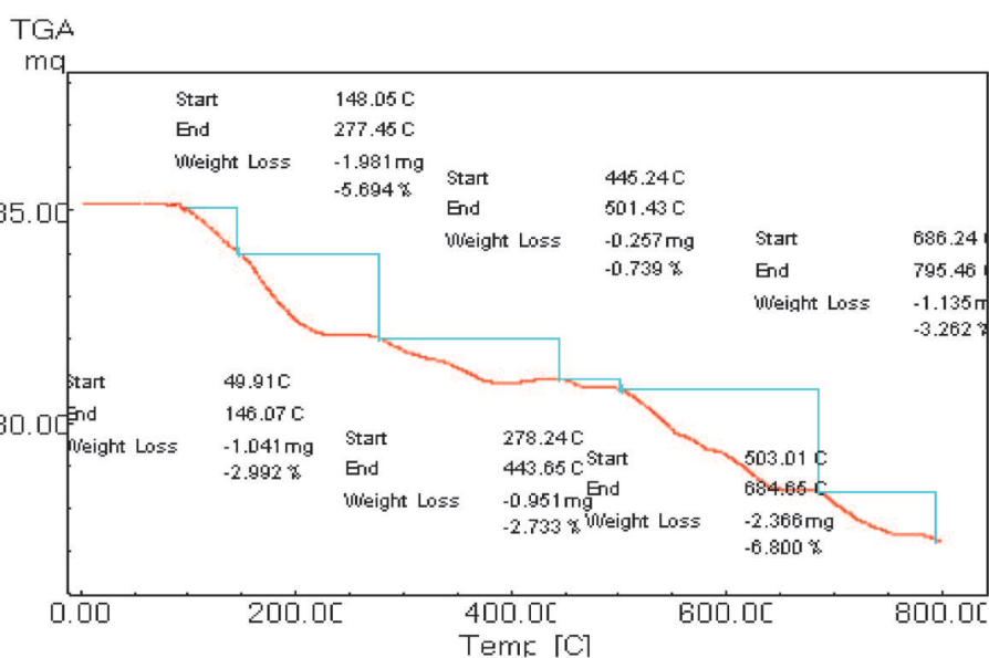
Figure 4. TGA thermogram for R1
