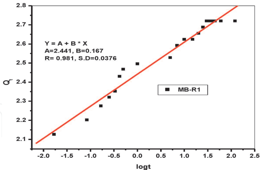
Figure 10. Elovich model kinetic plot for the sorption of MB onto the synthesized sorbents R1.
