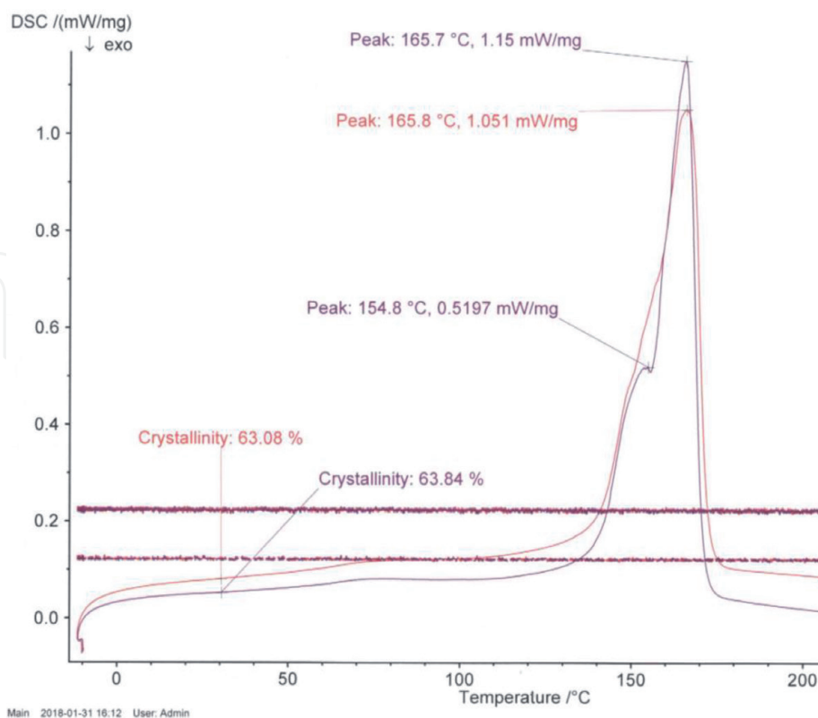
Figure 2. DSC dependencies for non-degraded blue bio PP, 3.5 EP, (red color) and blue bio PP, 3.5 EP, kept 42 days continuously in water.
