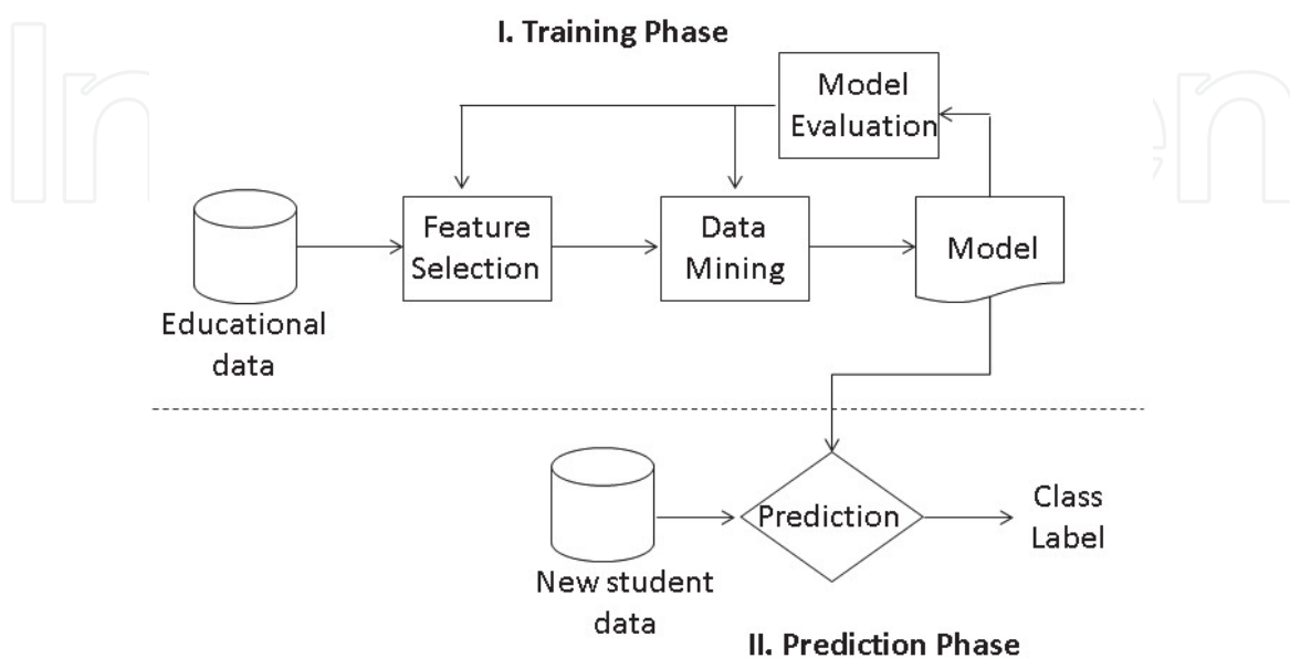
Figure 1. Flowchart of the data mining model.
