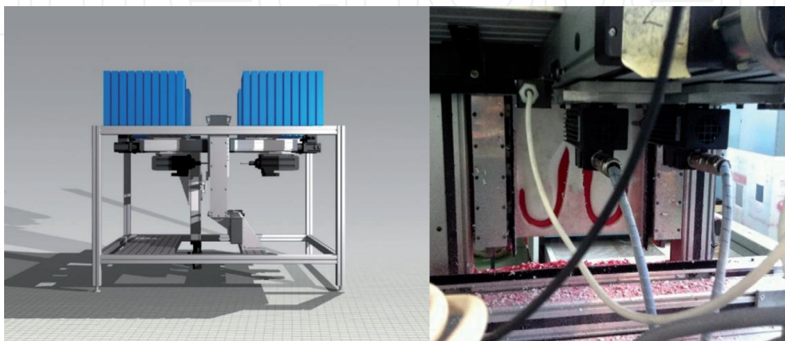
Figure 16. IPASIOU system.
