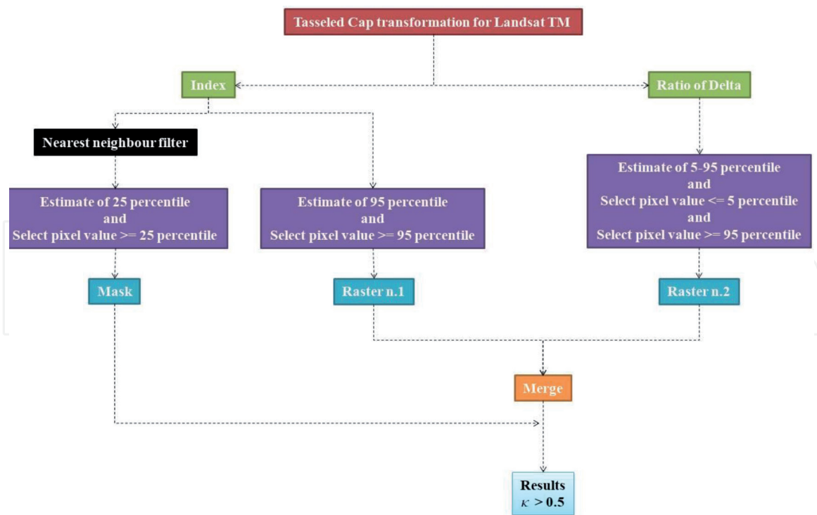
Figure 4. Operational workflow for illegal waste burial detection.
