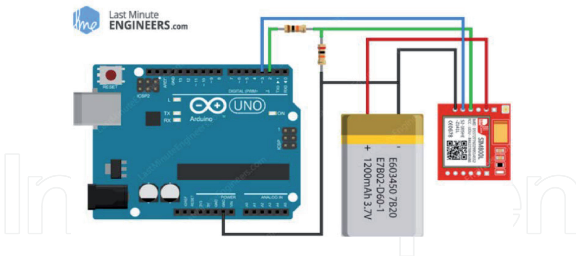
Figure 16. Circuit assembly for GSM module.
