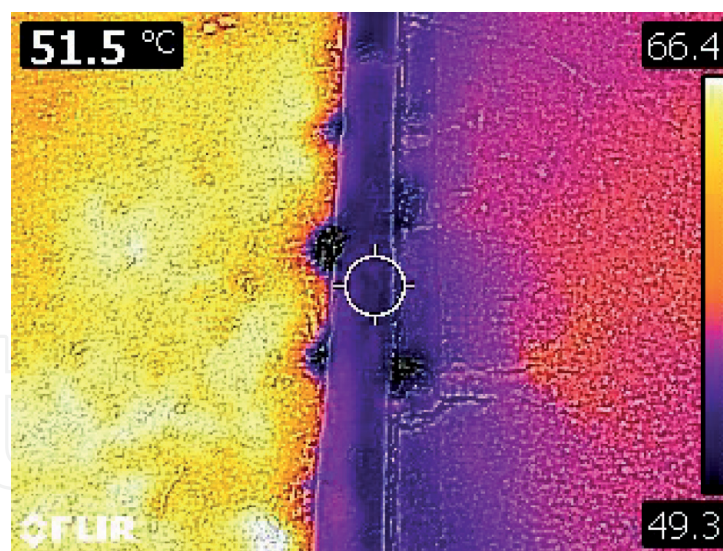
Figure 13. Asphalt (left) vs. concrete (right) temperatures ( ^{\circ}\text{C} ).
