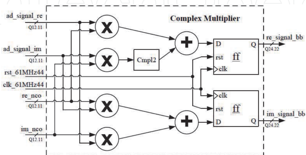
Figure 9. Architecture of the complex multiplier unit.
