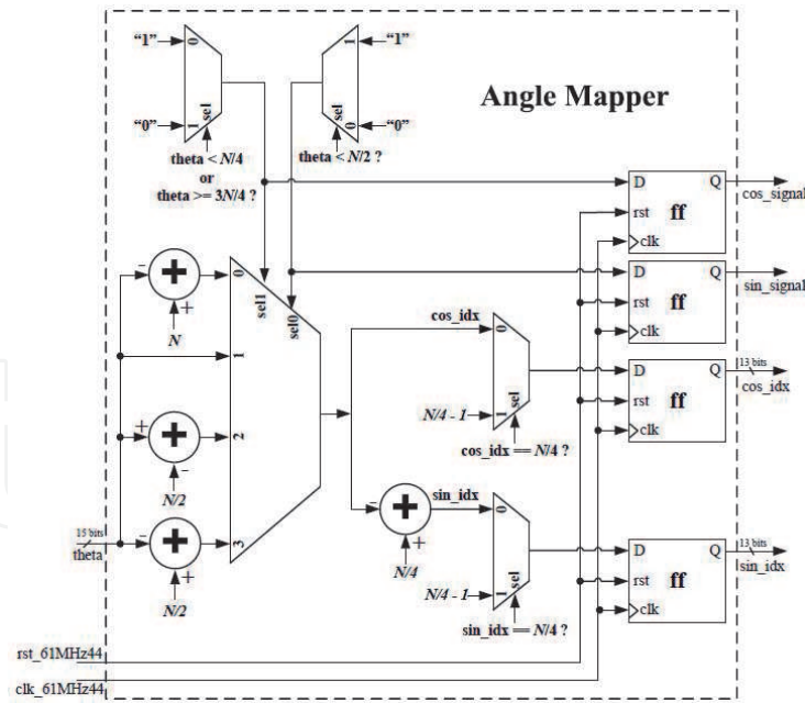
Figure 7. Architecture of the angle mapper unit.
