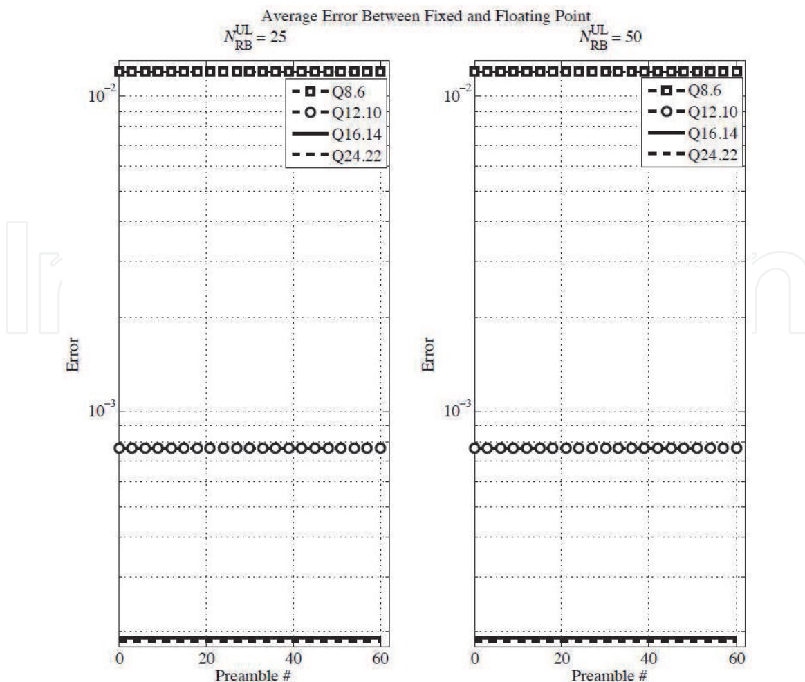
Figure 14. Average error between GM and DUT.
