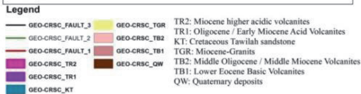
Figure 10. The geology cross-section of Jabal Sabir to Al-Hawban (the source of basic map [19]).
