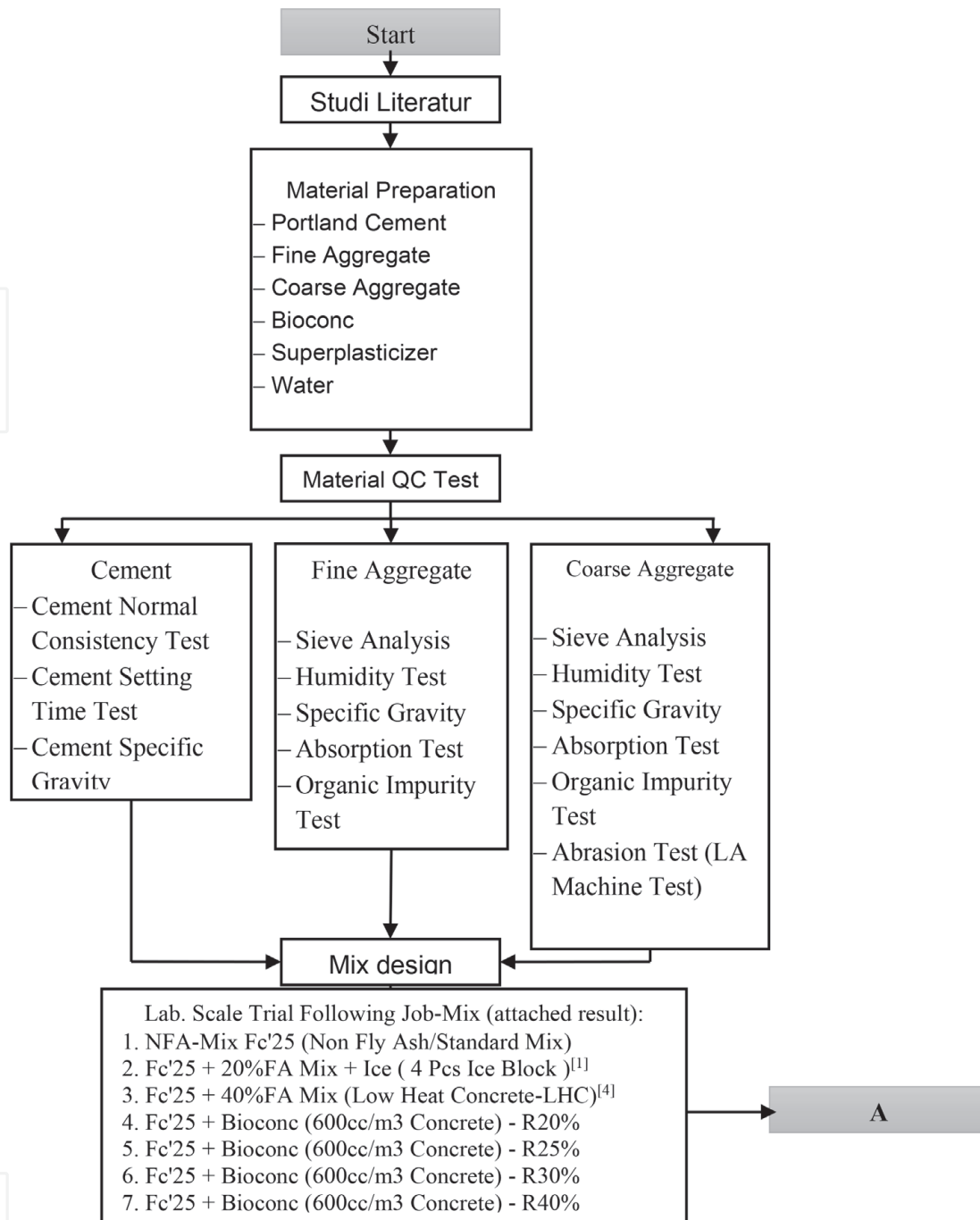
Figure 9. Flow chart of lab scale trial mix.
