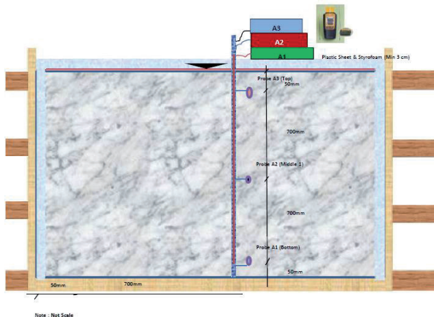
Figure 21. Thermocouple Fc'25 + FA40%-LHC graph monitoring, Summary Data & Mock-up Sketch.
