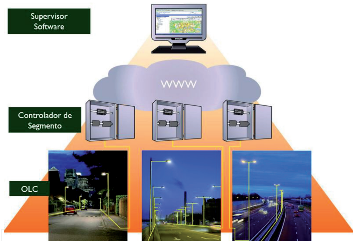
Figure 9. Point-to-point control system.
