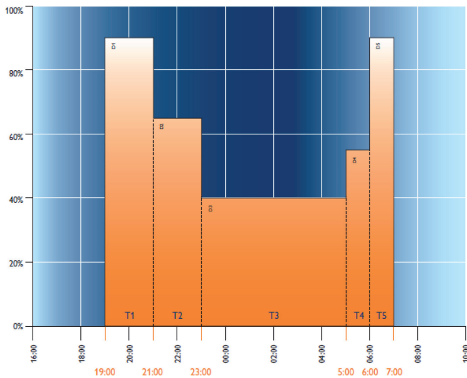
Figure 5. Dimming curve.
