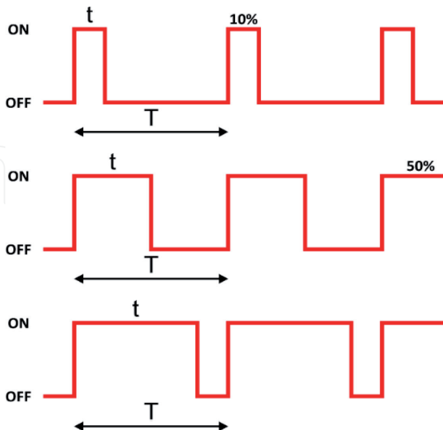
Figure 2. PWM regulation.
