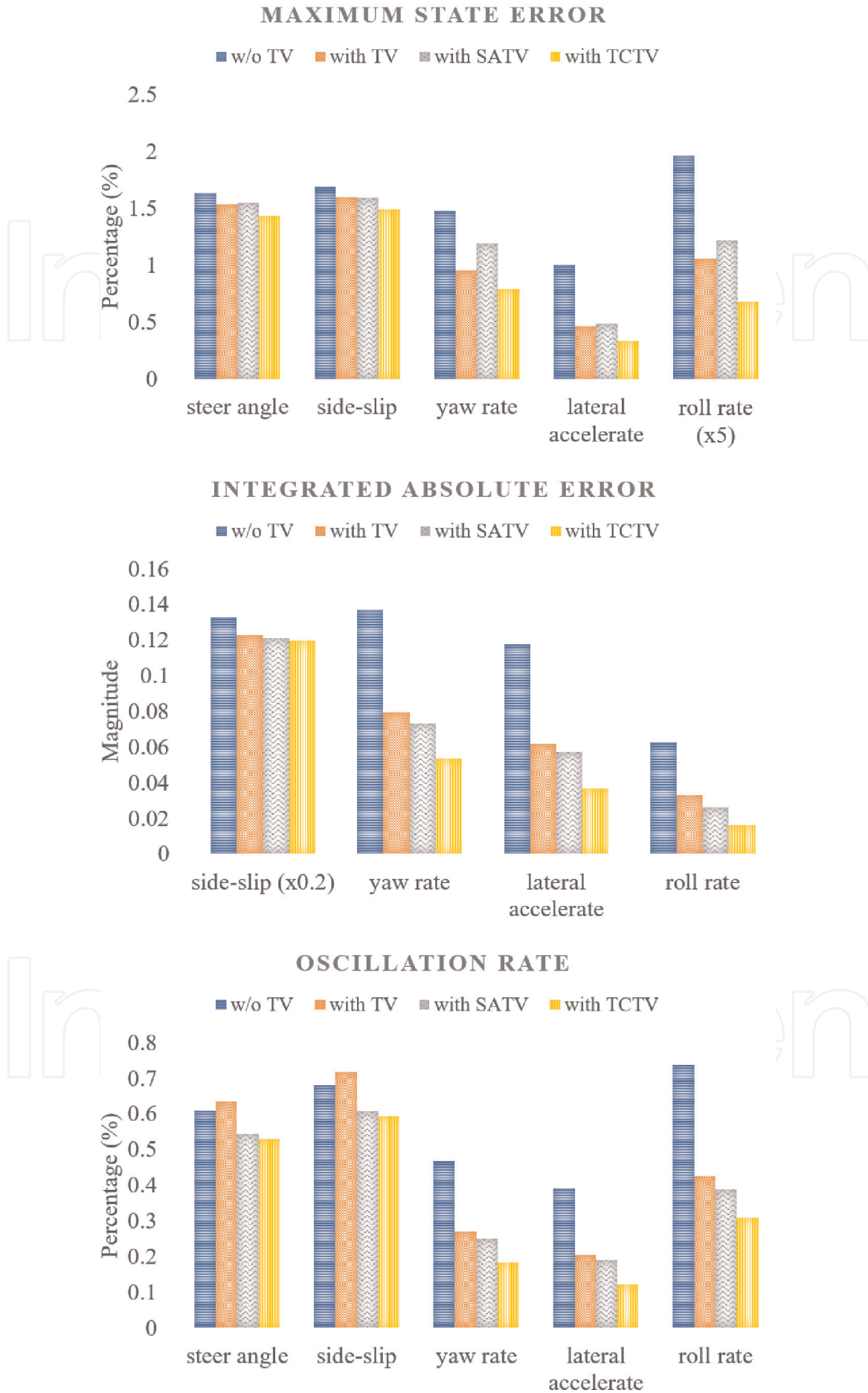
Figure 26. The performance indices comparison among different torque controllers when accelerating in a turn.
