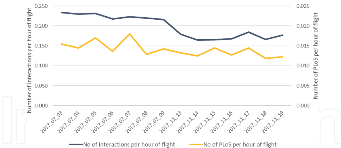
Figure 6. Number of aircraft interactions and PLoS per hour of flight.
