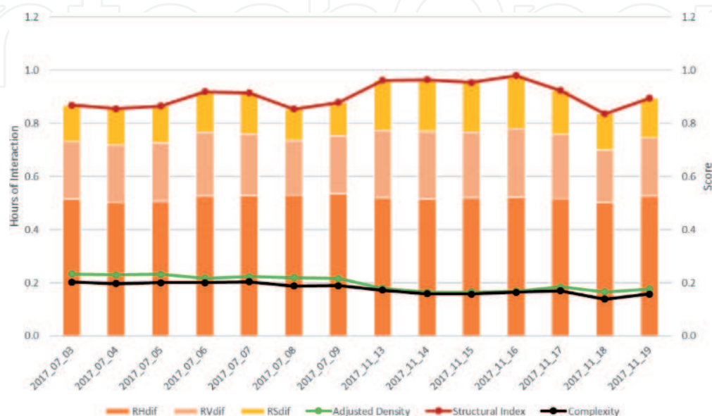
Figure 5. Complexity parameters.
