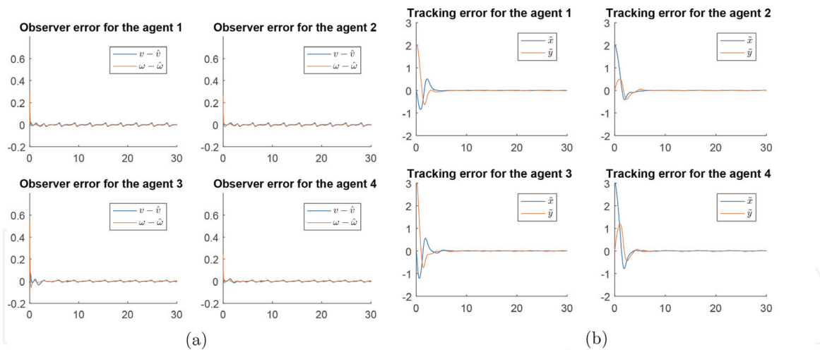
Figure 7. Observer errors and tracking errors using observer-based controller. (a) Observer errors using observer (13) and (14). (b) Tracking errors using controller (38) with (17).
