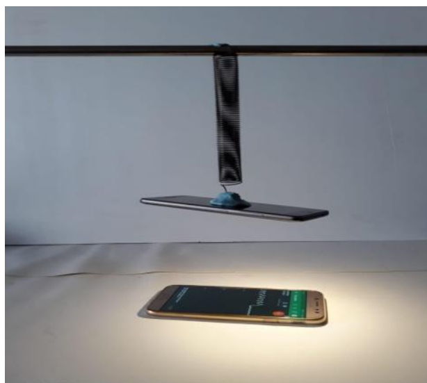
Figure 1. The photography of the basic apparatus, comprised of a spring pendulum with an oscillating smartphone as the actual mass and a stationary second smartphone.
