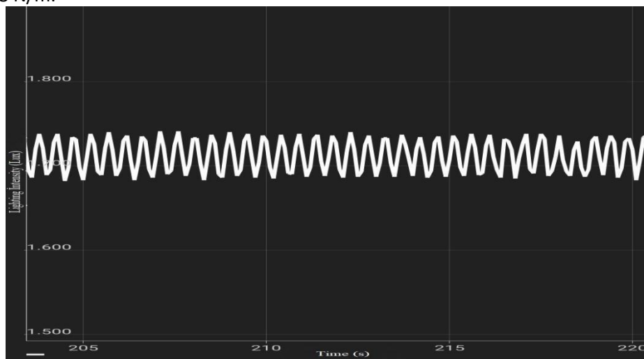
Figure 4. The oscillation screenshot of the second spring, noticeably showing the simple harmonic motion of the spring –mass system.
