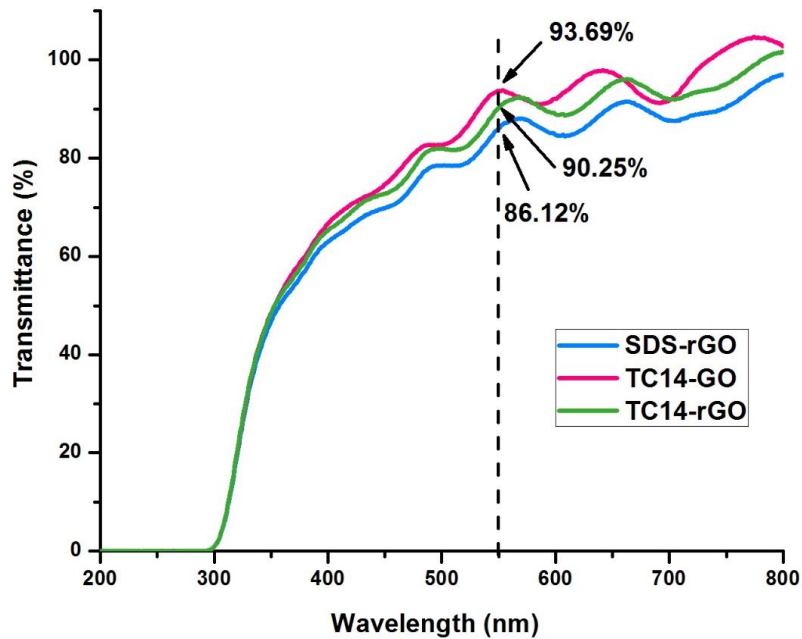
Fig. 3. The transmittance of fabricated GO and rGO thin films by TC14 and SDS surfactants.
