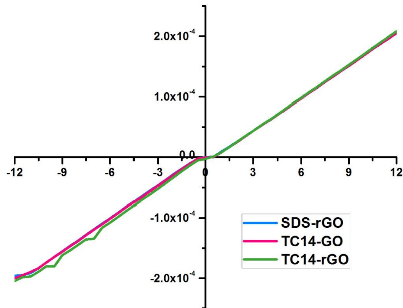
Fig. 4. The electrical resistivity based on I - V measurement of fabricated GO and rGO thin films by TC14 and SDS surfactants.
