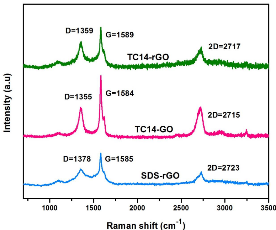
Fig. 2. Micro-Raman spectra of fabricated GO and rGO thin films by TC14 and SDS surfactants.
