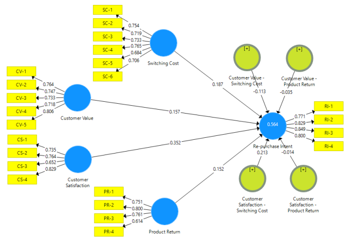
Figure 2. Result of PLS Path Model
