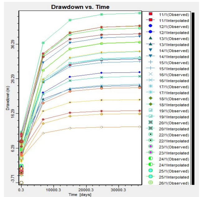
Figure 8. Drawdown Vs time at Q_{out}/Q_{in} = 370\%
