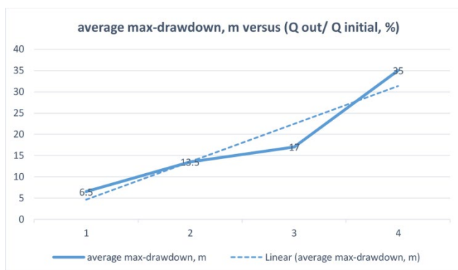
Figure 9. Average max- drawdown, m VS ( Q_{out}/ Q_{recharge} )
