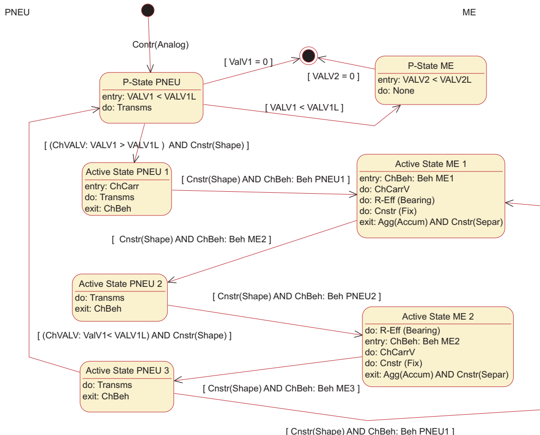
Fig. 4: Description of a structure of principles from Fields of Activities PNEU and ME by State diagram
