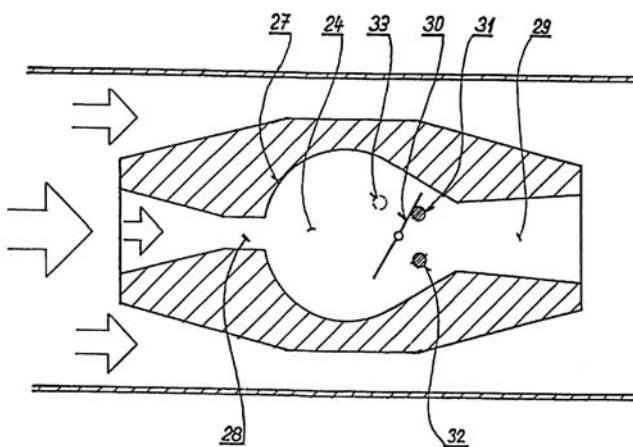
Fig. 5: One possible interpretation of solution x of the conceptual redesign problem from Example 1. (Description: 30 ... flapper, 31 , 32 , 33 ... constraint pins, 28 , 29 ... input and output neck, 24 ... interaction space, 27 ... shaped wall of the interaction space)
