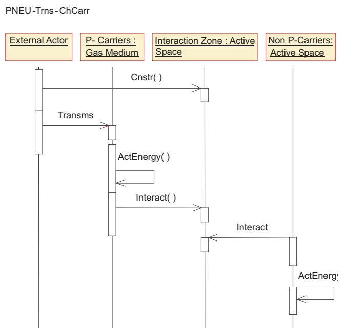
Fig. 3: Sequence diagram for principle “PNEU – Trns – CHCarr”
