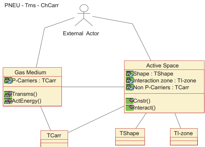
Fig. 2: Class diagram for principle “PNEU – Trns – CHCarr”
