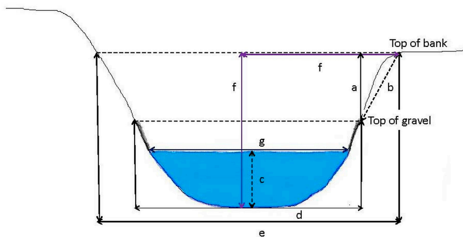
Figure 6. Cross-section view of channel and bank dimensions measured during a rapid physical habitat assessment (rPHA): (a) bank height; (b) bank slope; (c) thalweg depth; (d) channel width; (e) bankfull width; (f) relative thalweg depth (vertical) and thalweg position (horizontal); and (g) wetted width.
