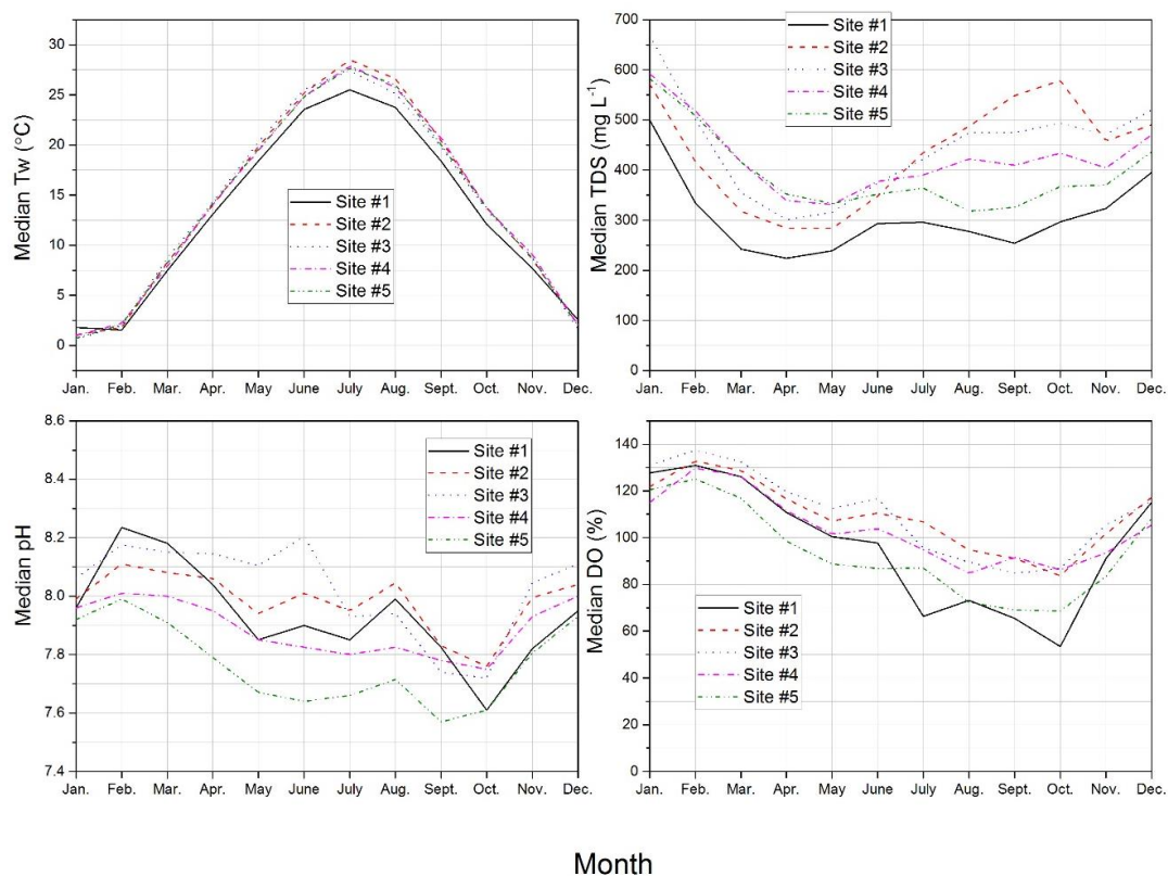
Figure 8. Median monthly water temperature ( T_w ) ( ^{\circ}\text{C} ), total dissolved solids (TDS) ( \text{mg L}^{-1} ), pH, and dissolved oxygen (%) at each gauging site ( n = 5 ) during study period (October, 2010–May 2014) in Hinkson Creek Watershed, MO, USA.
