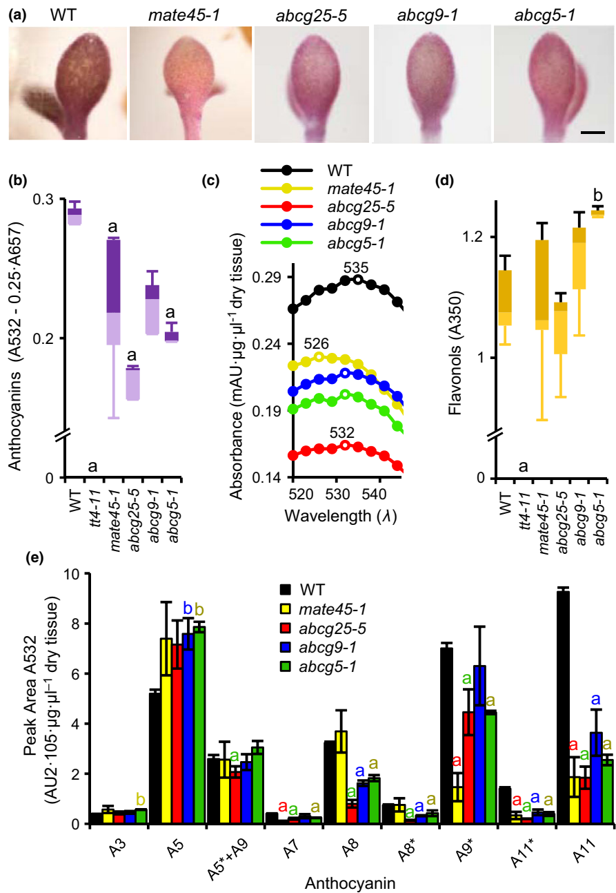
FIGURE 1 A high-throughput screen identifies metabolite transporter genes involved in the anthocyanin response to anthocyanin induction condition (AIC) stress. (a) Pale anthocyanin pigmentation phenotypes of the four transporter mutants when grown under AIC condition. The mutants mate45-1 (CS865060), abcg25-5 (SALK_128873C), abcg9-1 (SALK_045397C), and abcg5-1 (SALK_074250C) had pink cotyledon color, whereas the wild-type (WT) had purple cotyledons. 24-well multi-titer plates were incubated on a rotary shaker under 24 hr light for 5 days. (b) Total anthocyanin absorbance of methanolic extracts. tt4-11 is a flavonoid biosynthesis mutant. Error bars represent the standard error of the mean ( n = 3 ). a Less than control, b greater than control, p < 0.05 ; two-tailed Student's t test. (c) Spectral scan of methanolic extracts in the absorbance range of anthocyanins. Open circles and numbers above curves indicate absorbance maxima. (d) Total flavonol absorbance of methanolic extracts. (e) Relative anthocyanin amounts in methanolic extracts determined by HPLC-PDA
