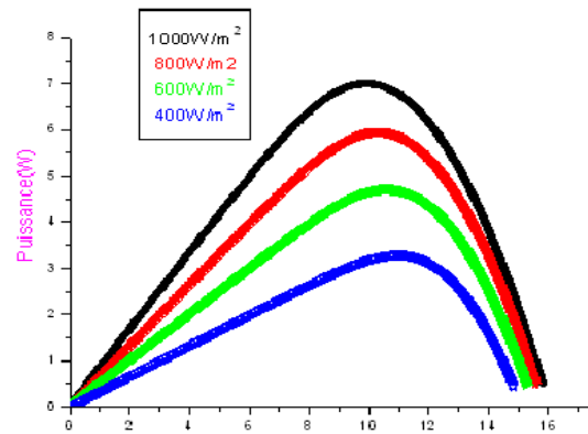
Fig.7: The influence of illumination on the characteristic P (V) for the panel tandem
