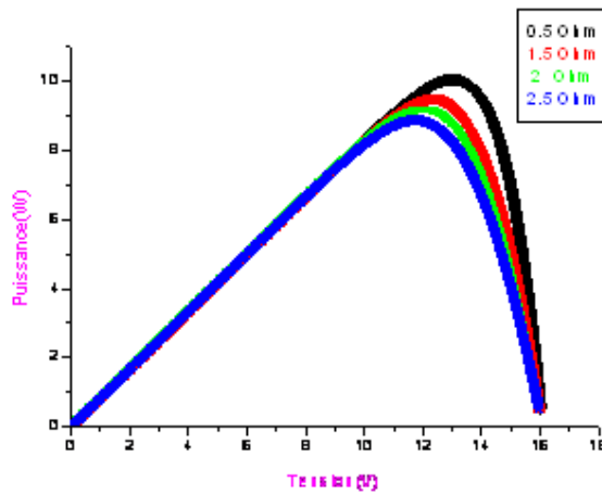
Fig.11: the influence of the series resistance on the characteristic P (V) for the panel tandem
