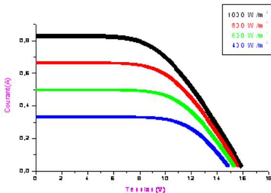
Fig.6: The influence of illumination on the characteristic I (V)
