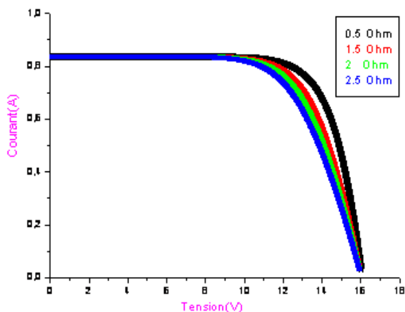
Fig.10: the influence of the series resistance on the characteristic I (V) for the panel tandem
