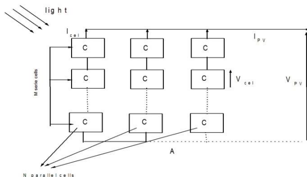
Fig. 2: Photovoltaic Panel
