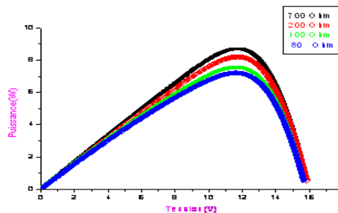
Fig.13: The influence of the series resistance on the characteristic P (V)
