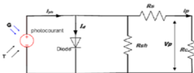
Fig 3 Equivalent circuit of a solar cell
