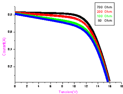
Fig.12: The influence of the series resistance on the characteristic P (V) for the panel tandem
