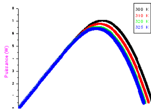
Fig.9: The influence of temperature on the characteristic P (V) for the panel Tandem
