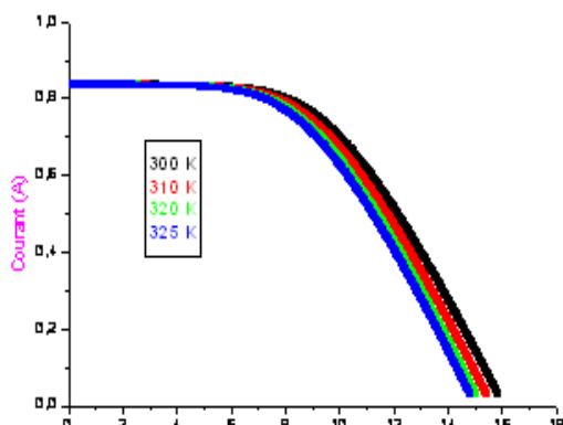
Fig.8: The influence of temperature on the characteristic I (V) for the panel Tandem
