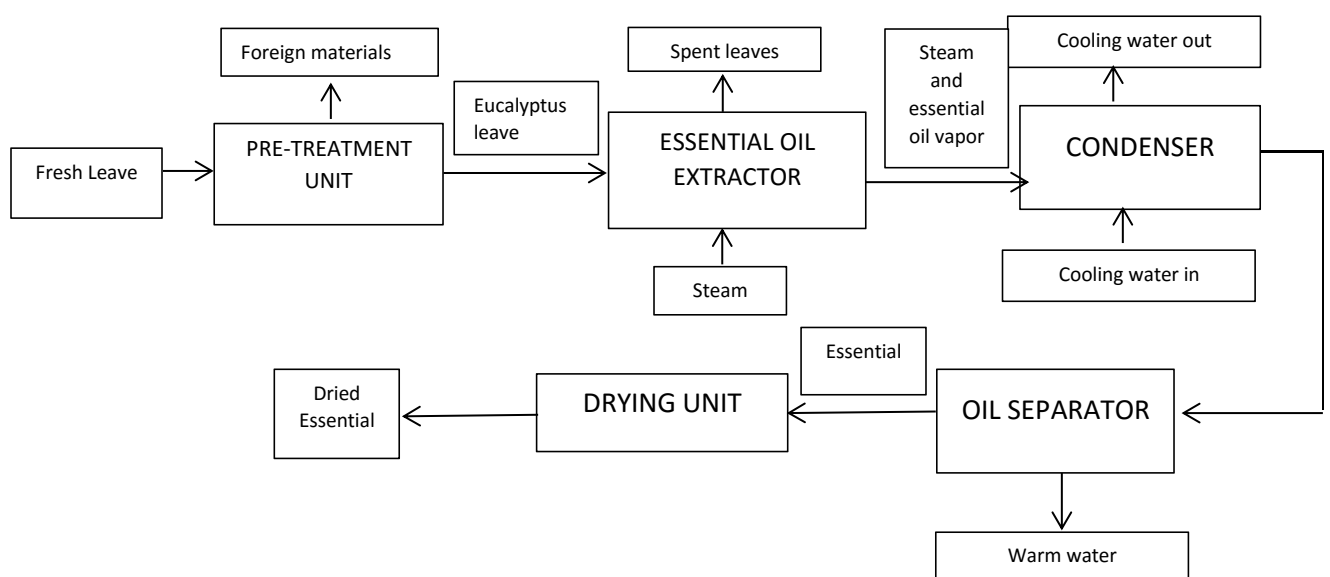
Figure 1: Block diagram for the steam extraction of essential oil from Eucalyptus leaves
