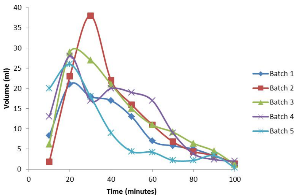
Figure 10: Extraction pattern of essential oil as a function of time
