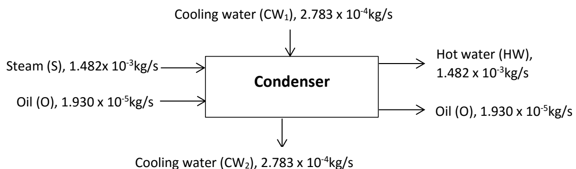
Figure 7: Material balance over oil condenser
