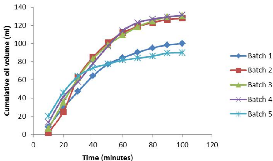
Figure 11: Cumulative volume of essential oil as a function of time
