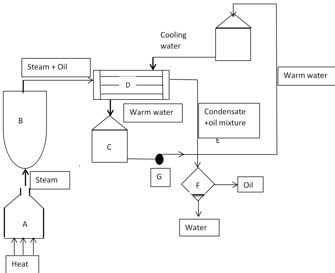
Figure 2: Flow sheet for the steam extraction of essential oil from Eucalyptus leaves
