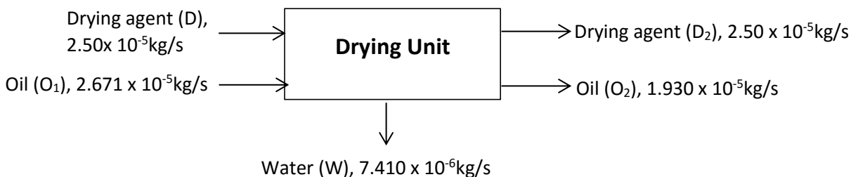
Figure 9: Material balance over drying unit
