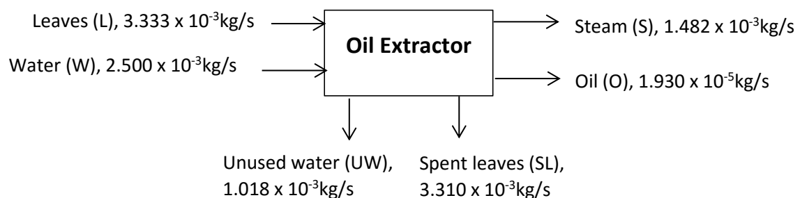
Figure 6: Material balance over oil extractor
