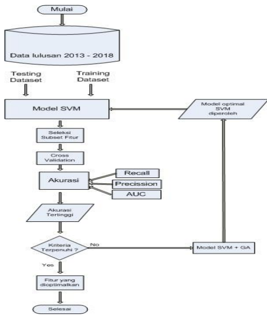
Figure 1. Activity Diagram of The Optimization Hybrid of Genetic Algorithm and Support Vector Machine
