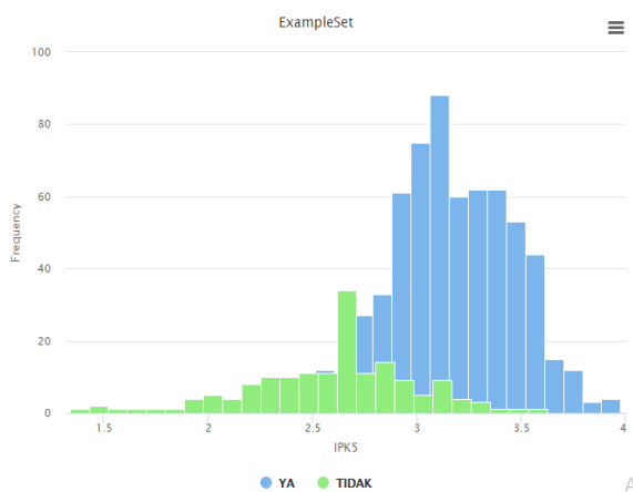
Figure 2 Student Graduation Diagram with SVM Method
