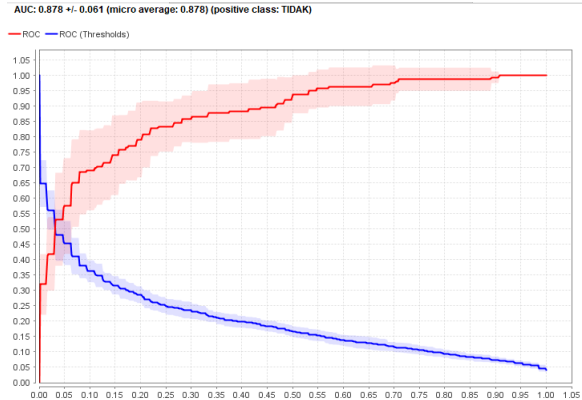
Figure 3 Area Under Curve (AUC) SVM
