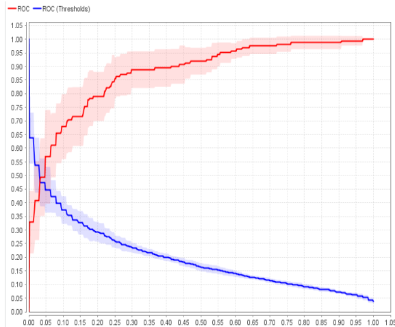
Source: (Ridwansyah, Wijaya, and Purnama 2020) Figure 4 Area Under Curve (AUC) Optimasi Hybrid GA
