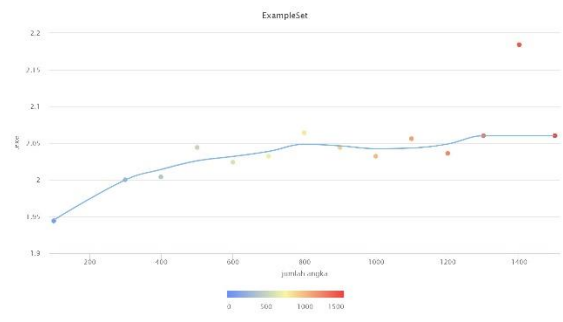
Source:(Iskandar et al., 2020) Figure 8. Scatter chart data is the amount of memory consumption bubble sort algorithm with Visual Studio 2010 extension EXE program.
