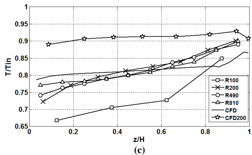
Figure 5.5 Comparison of the different grid resolutions of POMa and CFD (FLOVENT) model with a grid of 29 \times 27 \times 23 (a) Center pole; (b) East pole; (c) West pole
