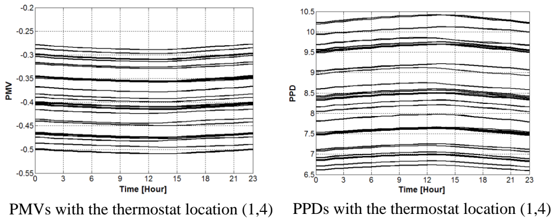
Figure 5.95 Zonal PMV and PPD profiles with the thermostat location (1,4) (Case 3)
