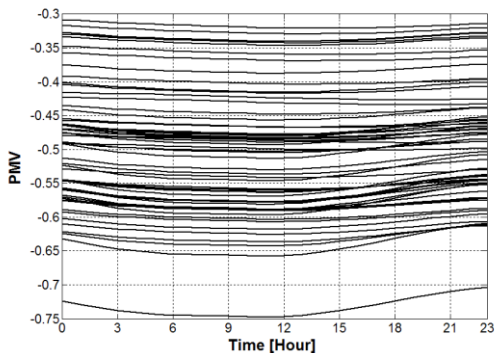
PMVs with the thermostat location (5,6)
