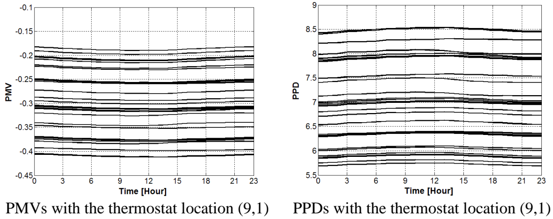
Figure 5.94 Zonal PMV and PPD profiles with the thermostat location (9,1) (Case 3)
