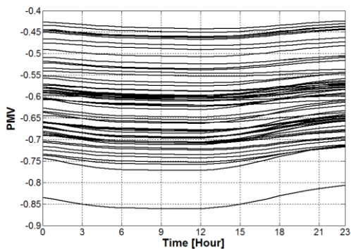
PMVs with the thermostat location (1,4)
