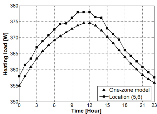
Figure 5.93 Heating loads of the original and integrated thermal models with the thermostat location (5,6) (Case 3)
