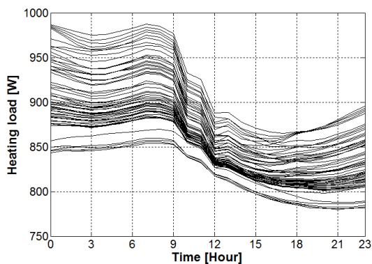
Figure 5.97 Heating loads with different thermostat locations (Case 4)
