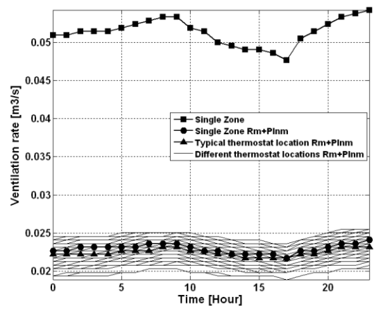
Figure 5.36 Supply airflow rate requirements of the case 1
