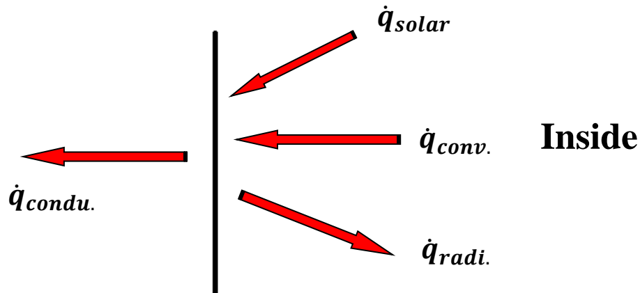
Figure 4.2 Room interior surface heat balance
