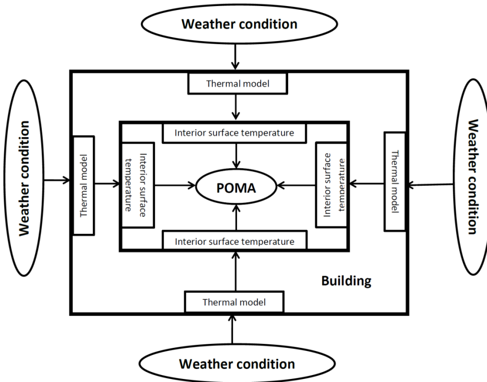
Figure 4.5 Integration of POMA and the thermal model
