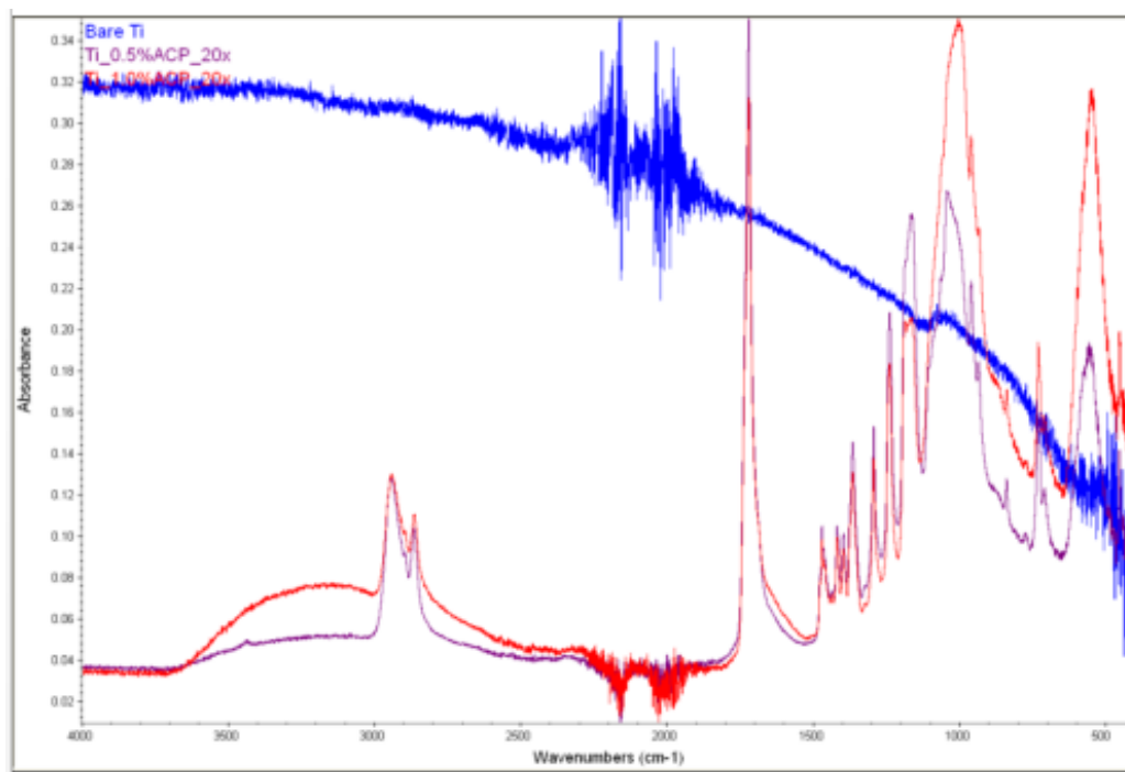
Figure A-1. Fourier transform infrared spectroscopy (FTIR) of bare Ti and polymeric coatings
